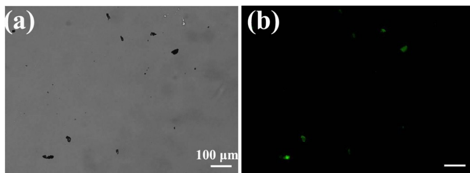
Figure S1 Dylight 488 fluorescently labeled PSS-graphene were analysed under (a) light scatter mode and (b) fluorescence mode.
