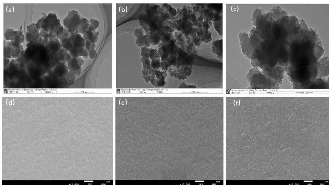
S1. TEM pictures of SA-g-AN copolymers a:SA/AN=1/8; b:SA/AN=1/11; c:SA/AN=1/14 and SEM of SA-g-AN film materials d:SA/AN=1/8; e:SA/AN=1/11; f:SA/AN=1/14
