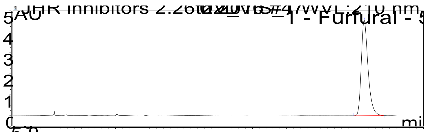
Fig. S1. Chromatogram of furfural solution isolated from hydrolyses.
