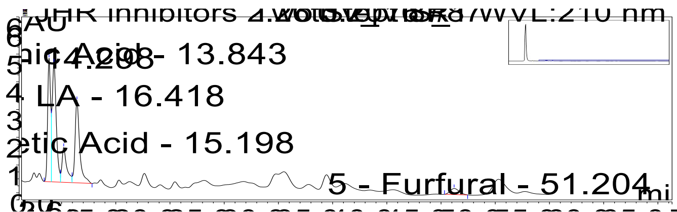
Fig. S2. Chromatogram of LA solution from hydrolyses.
