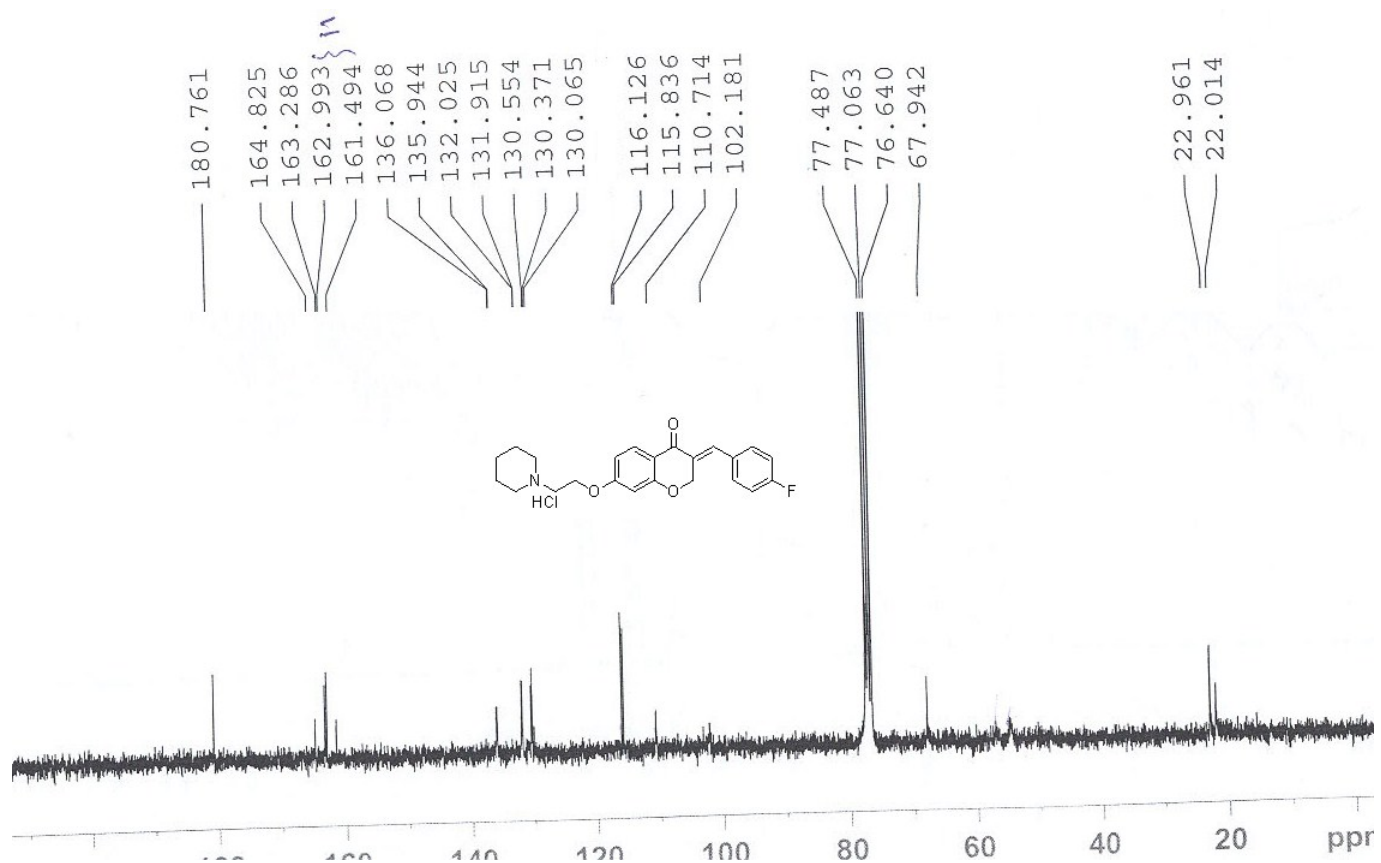
Fig. S16. ^{13}\text{C} NMR spectrum of product 8h
