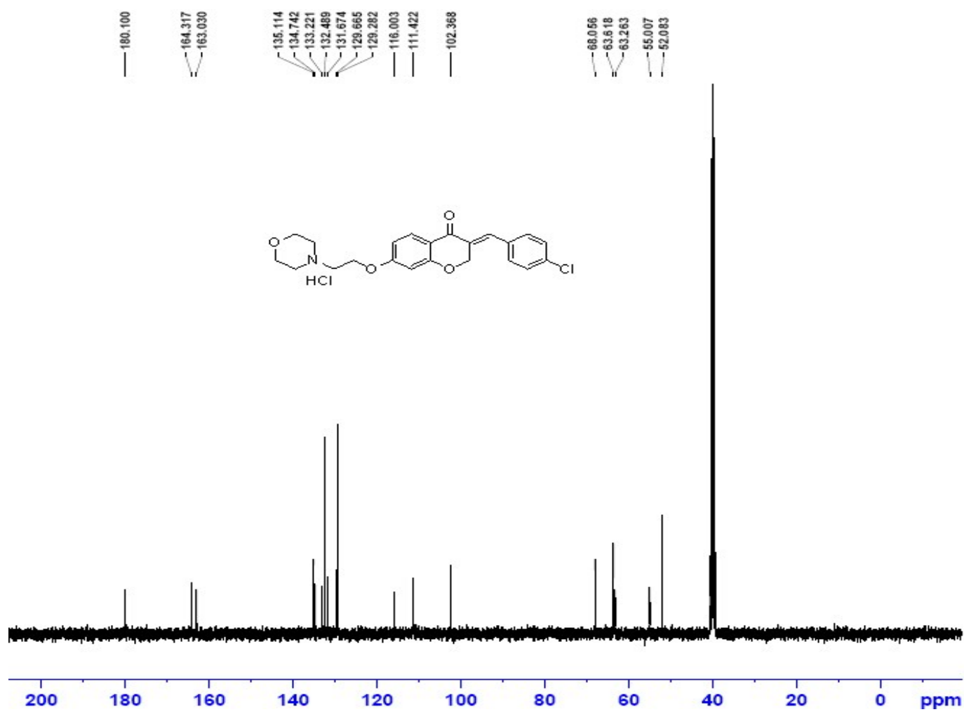
Fig. S6. 13 C NMR spectrum of product 8c
