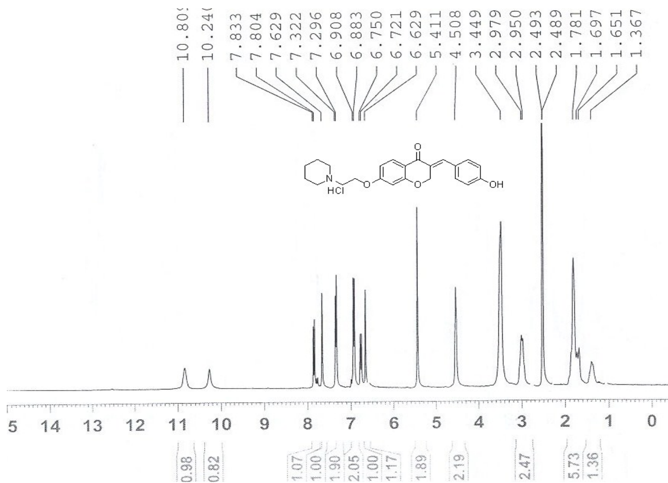
Fig. S20. 1 H NMR spectrum of product 8I
