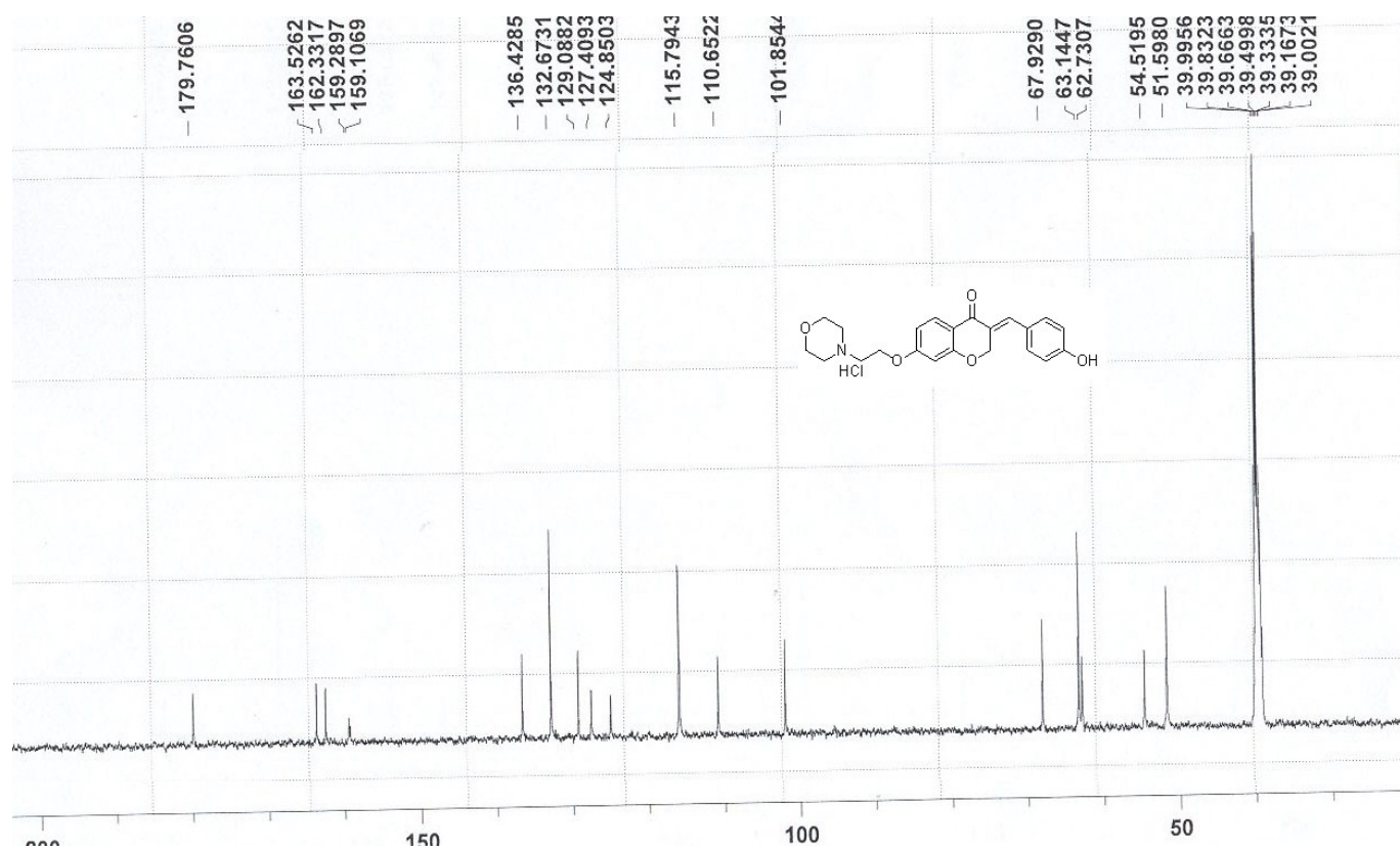
Fig. S12. 13 C NMR spectrum of product 8f
