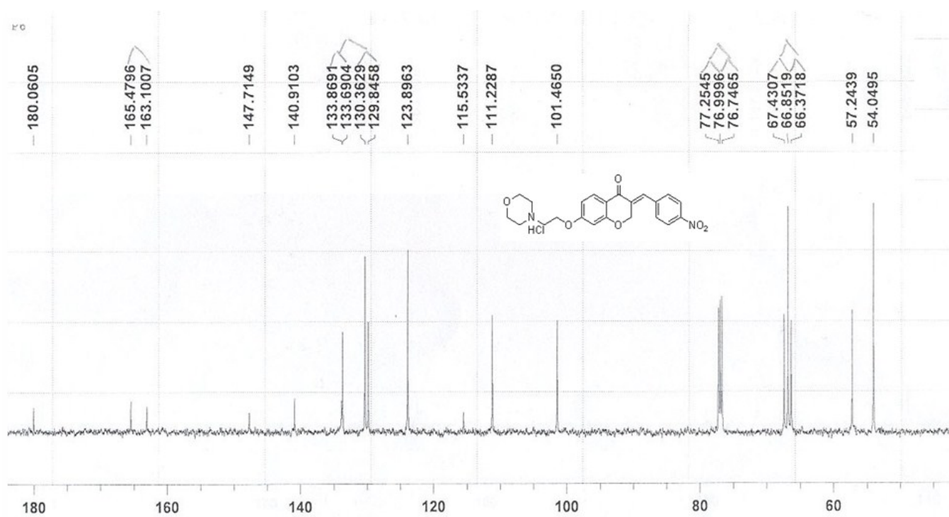
Fig. S2. ^{13}\text{C} NMR spectrum of product 8a
