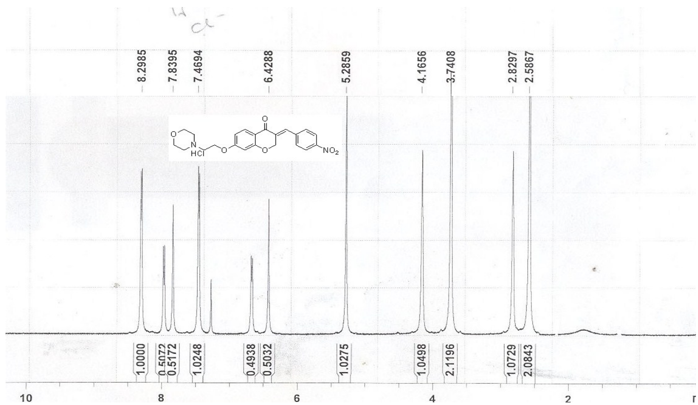
Fig. S1. 1 H NMR spectrum of product 8a
