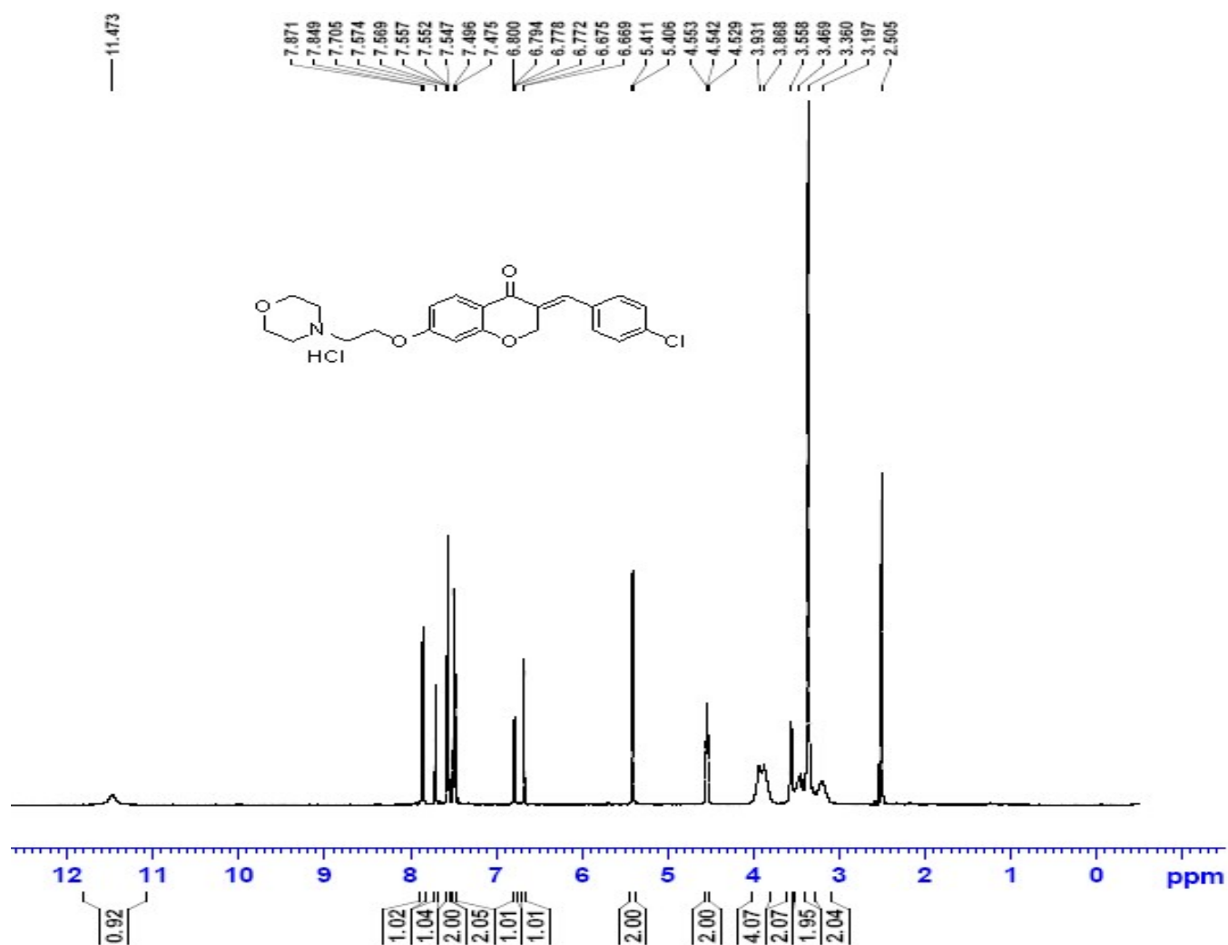
Fig. S5. 1 H NMR spectrum of product 8c
