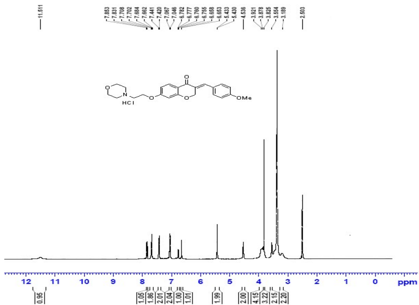
Fig. S7. ^1\text{H} NMR spectrum of product 8d
