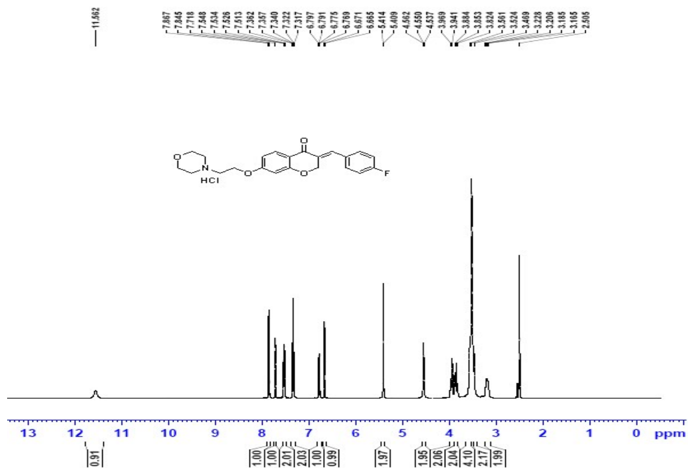
Fig. S3. 1 H NMR spectrum of product 8b
