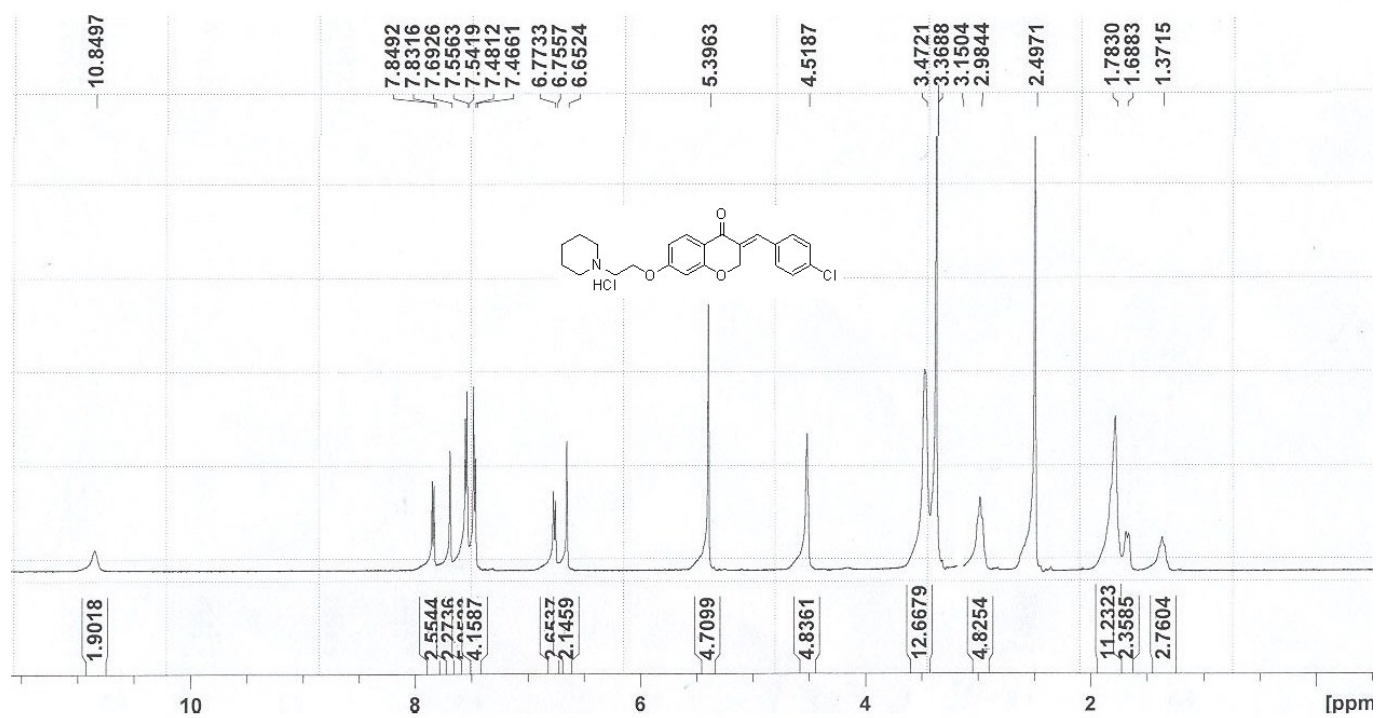
Fig. S17. 1 H NMR spectrum of product 8i
