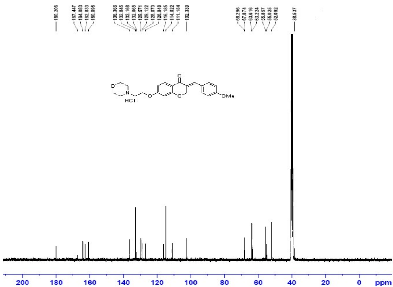
Fig. S8. 13 C NMR spectrum of product 8d
