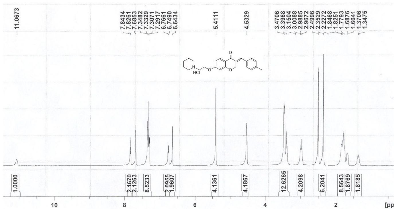
Fig. S19. 1 H NMR spectrum of product 8k
