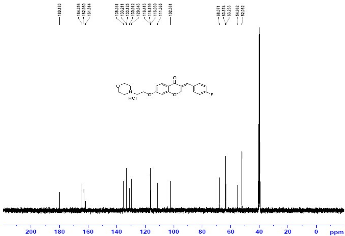
Fig. S4. ^{13}\text{C} NMR spectrum of product 8b
