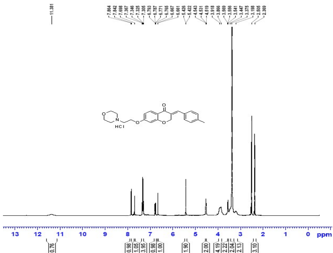
Fig. S9. 1 H NMR spectrum of product 8e
