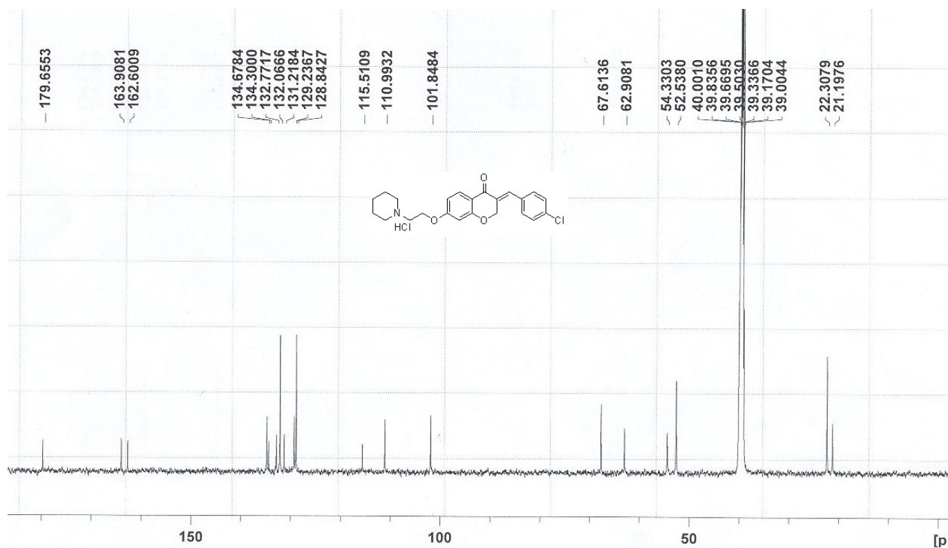
Fig. S18. 13 C NMR spectrum of product 8i
