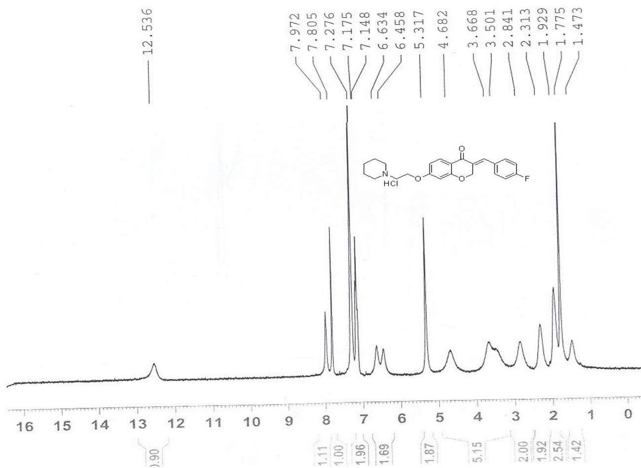
Fig. S15. 1 H NMR spectrum of product 8h
