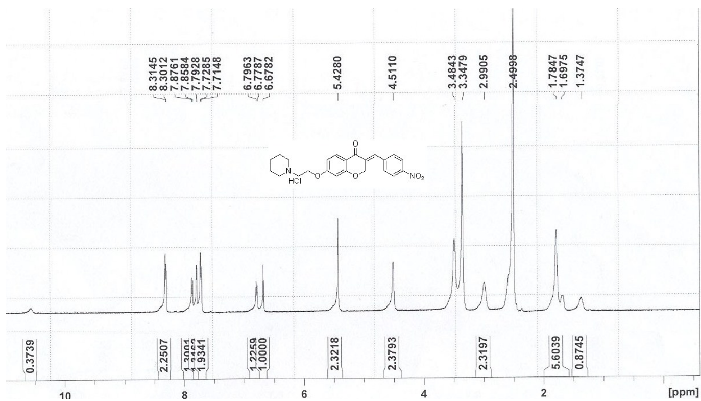
Fig. S13. 1 H NMR spectrum of product 8g
