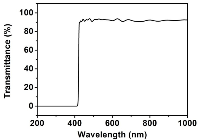
Fig. S2 Transmission spectra of the 420 nm long-pass filter.
