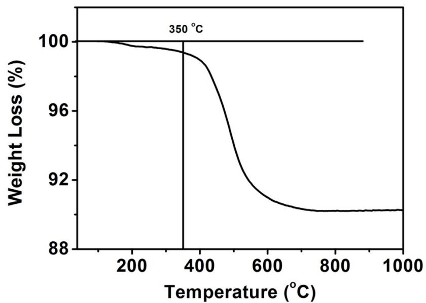
Fig. S3 TGA curve of the NYF@TiO 2 -3%Ag sample.
