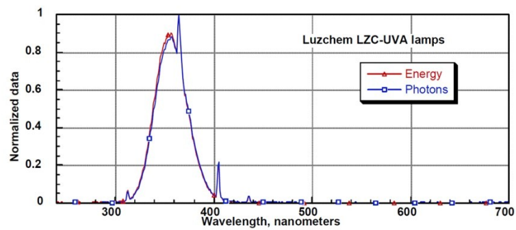
Fig. S1 Emission spectrum of LZC-UVA lamps.
