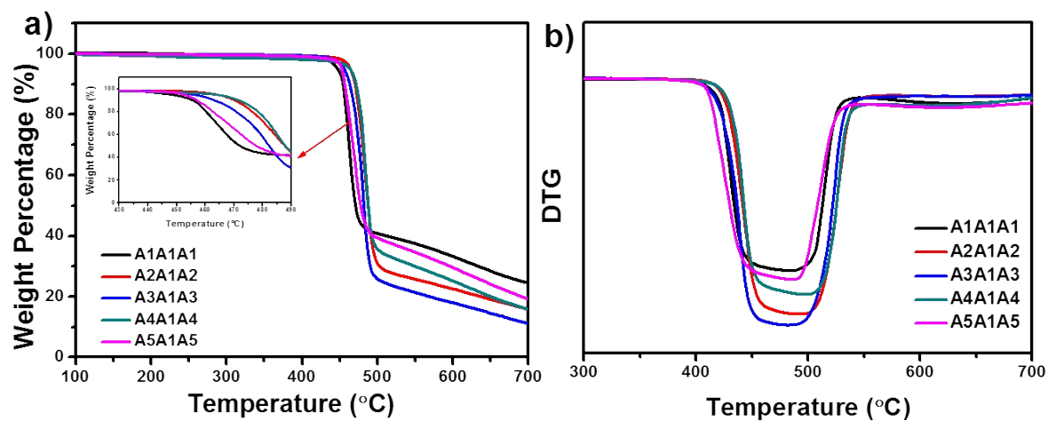
Fig. S2: TGA (a) and DTG (b) curves of sandwiched PVDF-HFP and its ZnO and Ni-doped ZnO nanocomposite films.
