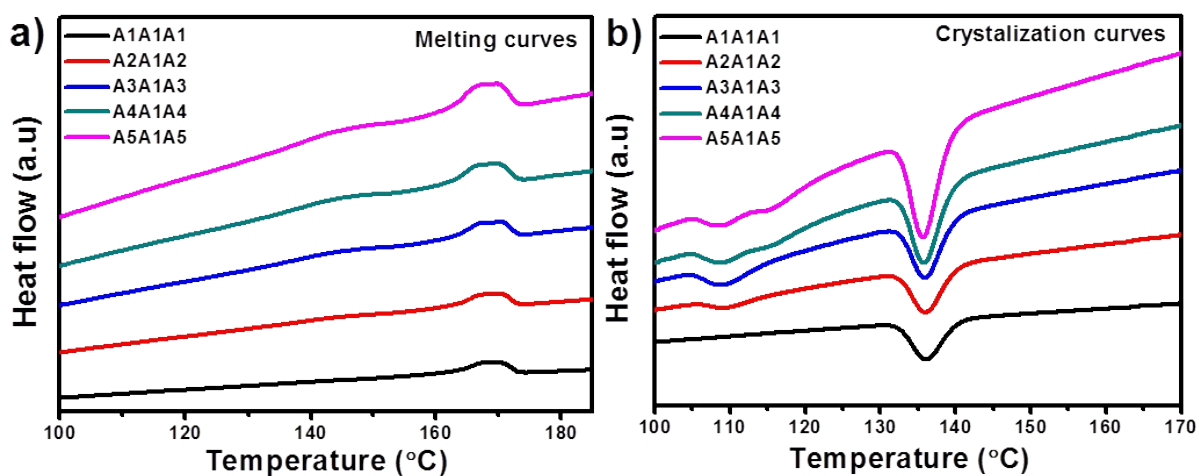
Fig. S1: DSC melting (a) and crystallization (b) curves of sandwiched PVDF-HFP and its nanocomposite films.
