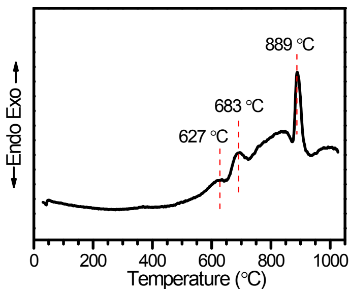
Figure S1 DTA curve of the 50SiO 2 -20Al 2 O 3 -29.95CaF 2 -0.05CrF 3 (in mol %) glass.
