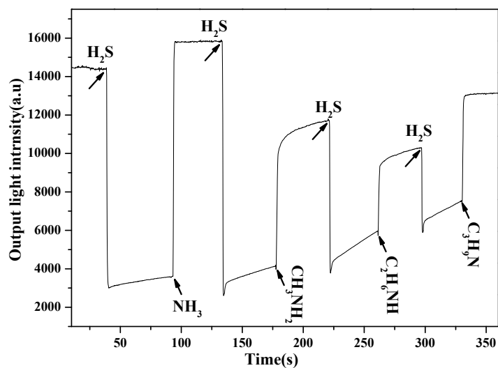
Figure S1. Response of protonated TPP thin film upon exposure to amine gases (100 ppm).
