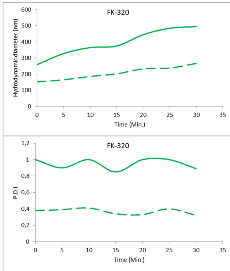
Fig. S2. Hydrodynamic diameter and polydispersity index of bare (solid line) and PNIPAM grafted (dashed line) FK320 SiNPs.
