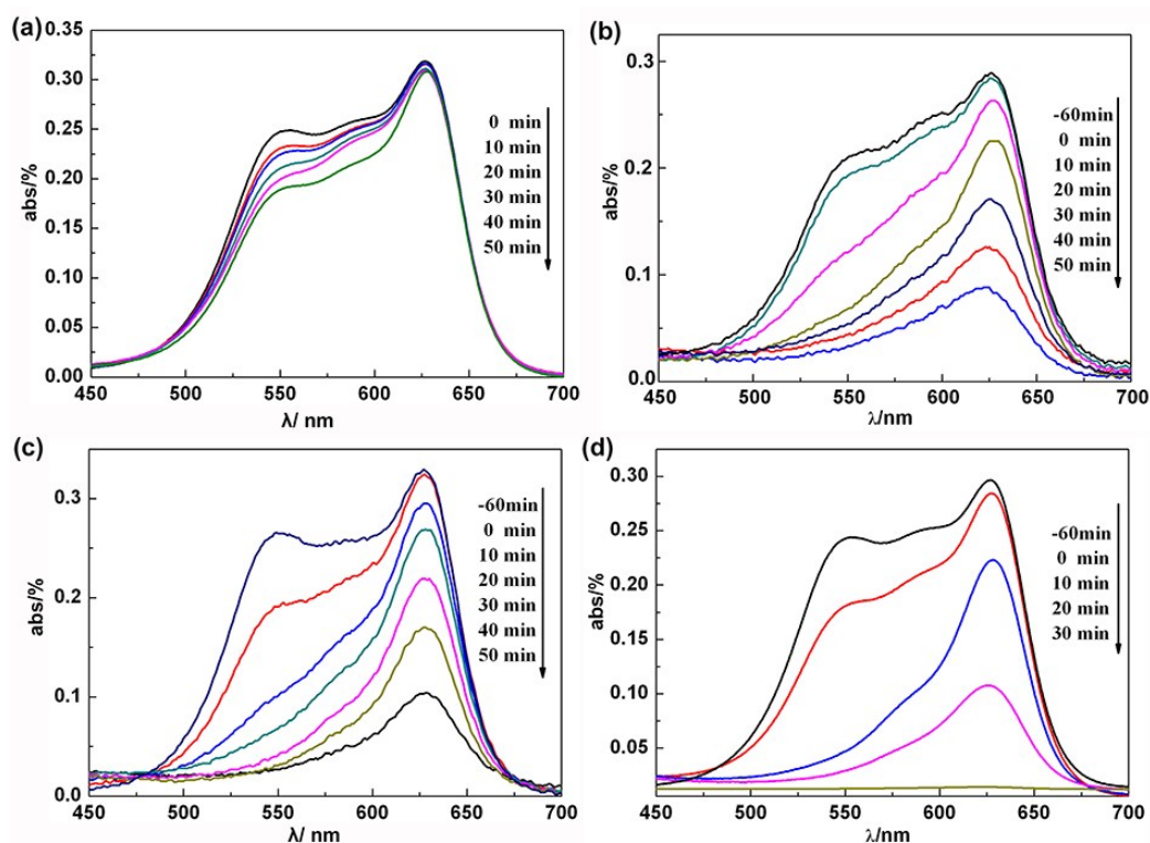
Fig. S1. The time-dependent absorption spectra of MB solution in the presence of (a) blank, (b) HZO (unanneal), (c) HZO (anneal) and (d) HZO@Gr.
