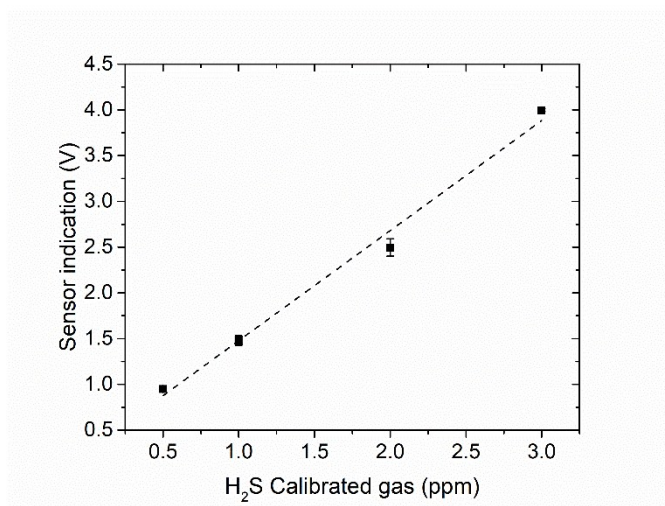
Fig. S1. Calibration of the electrochemical sensors by using precalibrated H 2 S gas mixtures.
