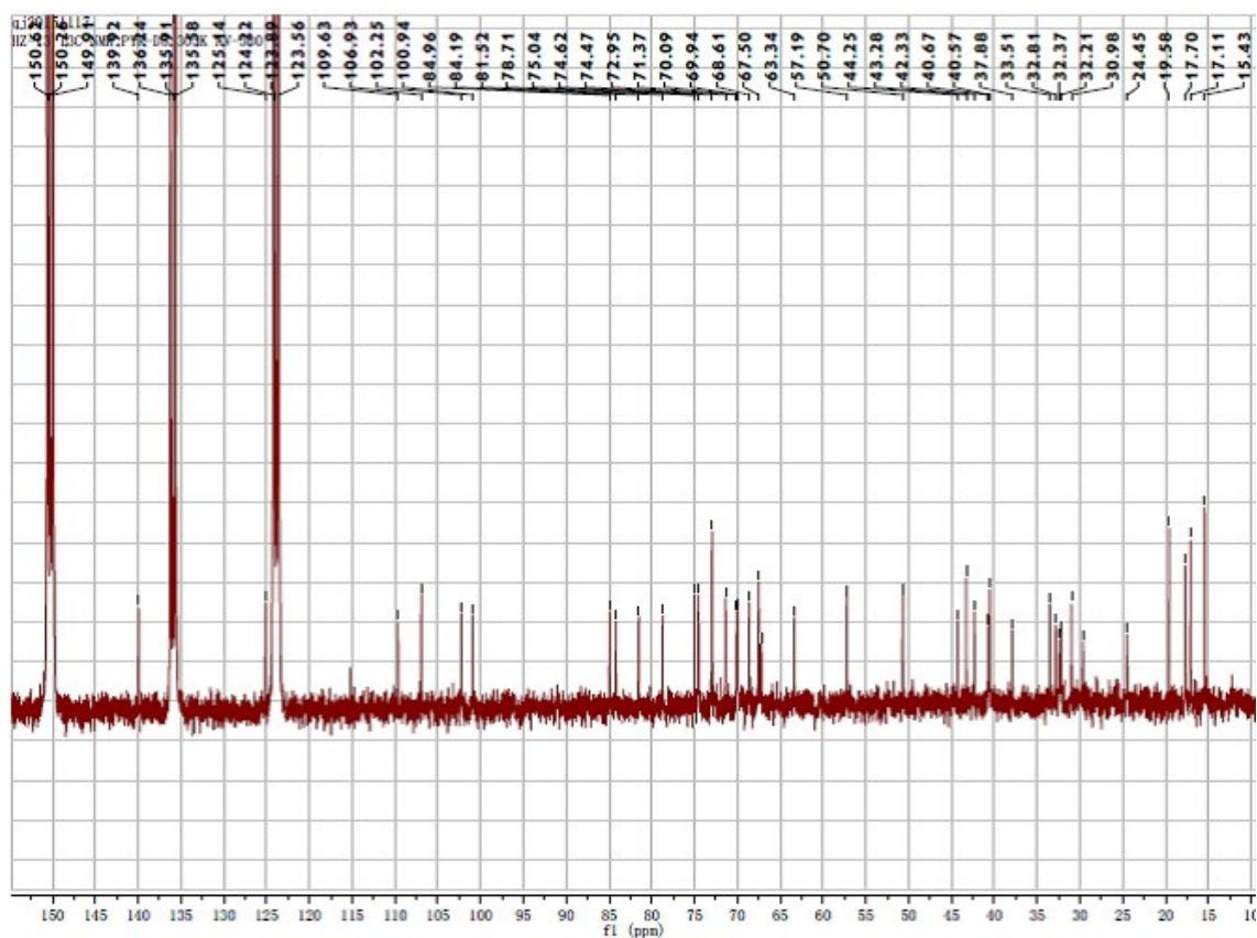
Figure S42. ^{13}\text{C} NMR spectrum of compound 7 (pyridine- d_5 )
