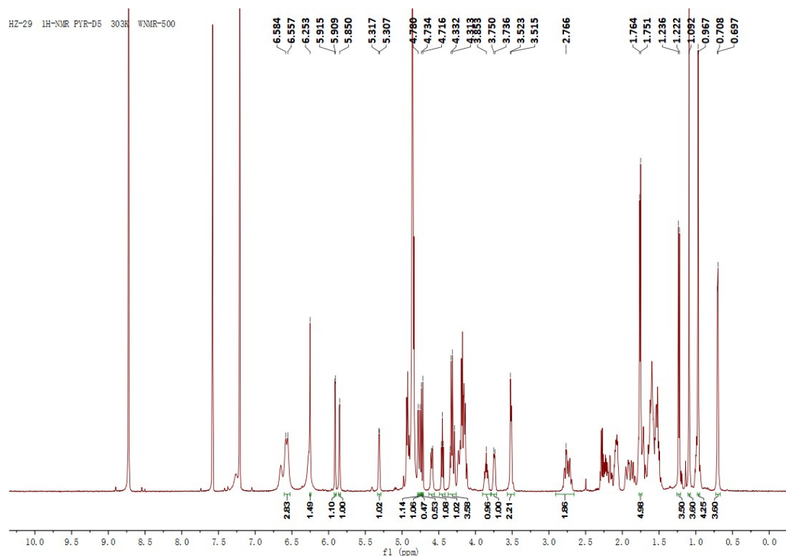
Figure S4. ^{13}\text{C} NMR spectrum of compound 1 (pyridine- d_5 )
