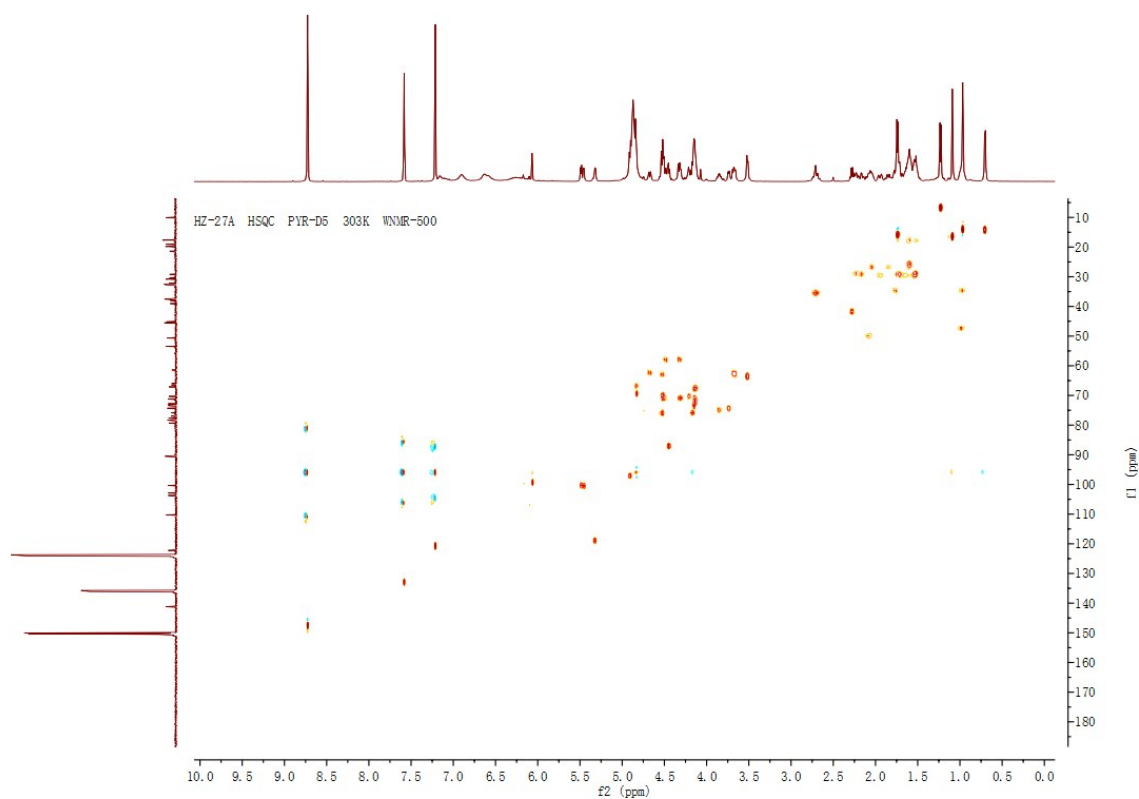
Figure S18. HSQC NMR spectrum of compound 3 (pyridine- d_5 )
