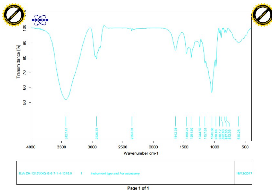
Figure S15. IR (KBr, disc) spectrum of compound 3
