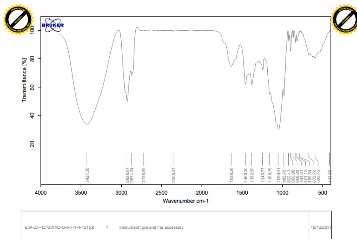
Figure S34. IR (KBr, disc) spectrum of compound 6
