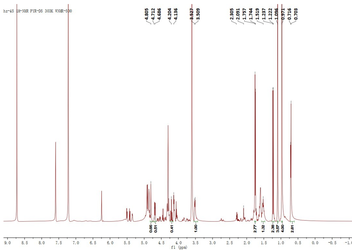
Figure S28. 1 H NMR spectrum of compound 5 (pyridine- d 5 )
