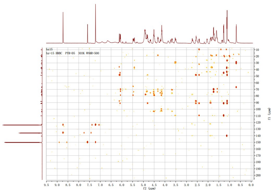
Figure S13. HMBC NMR spectrum of compound 2 (pyridine- d 5 )
