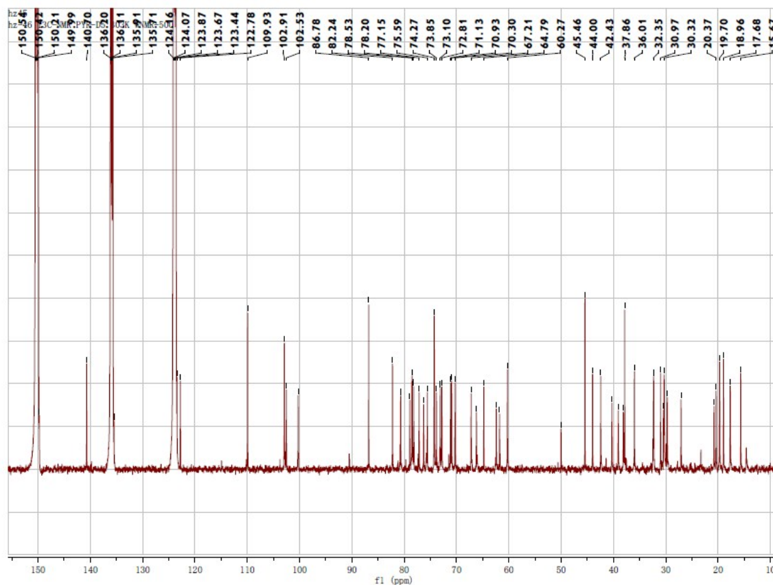
Figure S36. ^{13}\text{C} NMR spectrum of compound 6 (pyridine- d_5 )
