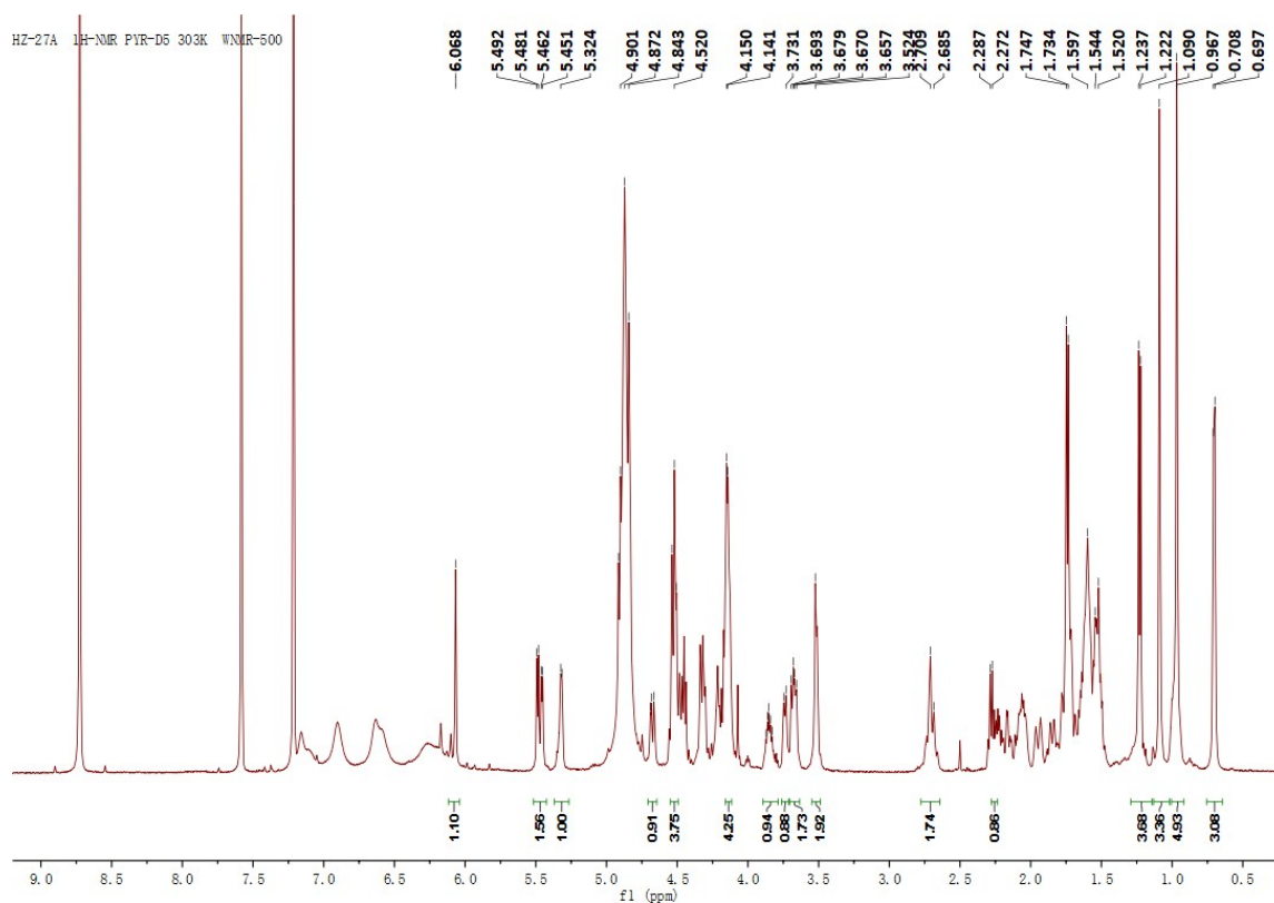
Figure S16. 1 H NMR spectrum of compound 3 (pyridine- d 5 )
