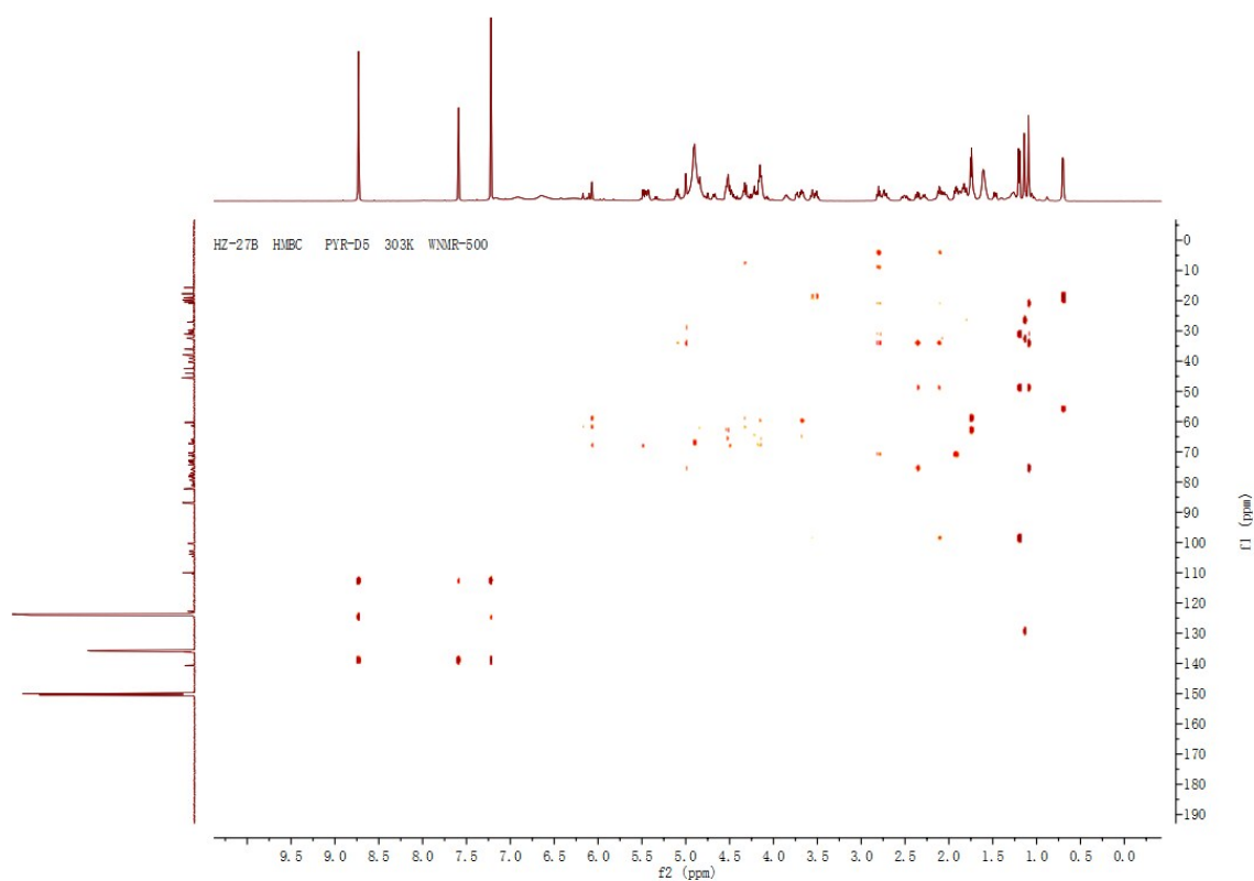
Figure S25. HMBC NMR spectrum of compound 4 (pyridine- d 5 )
