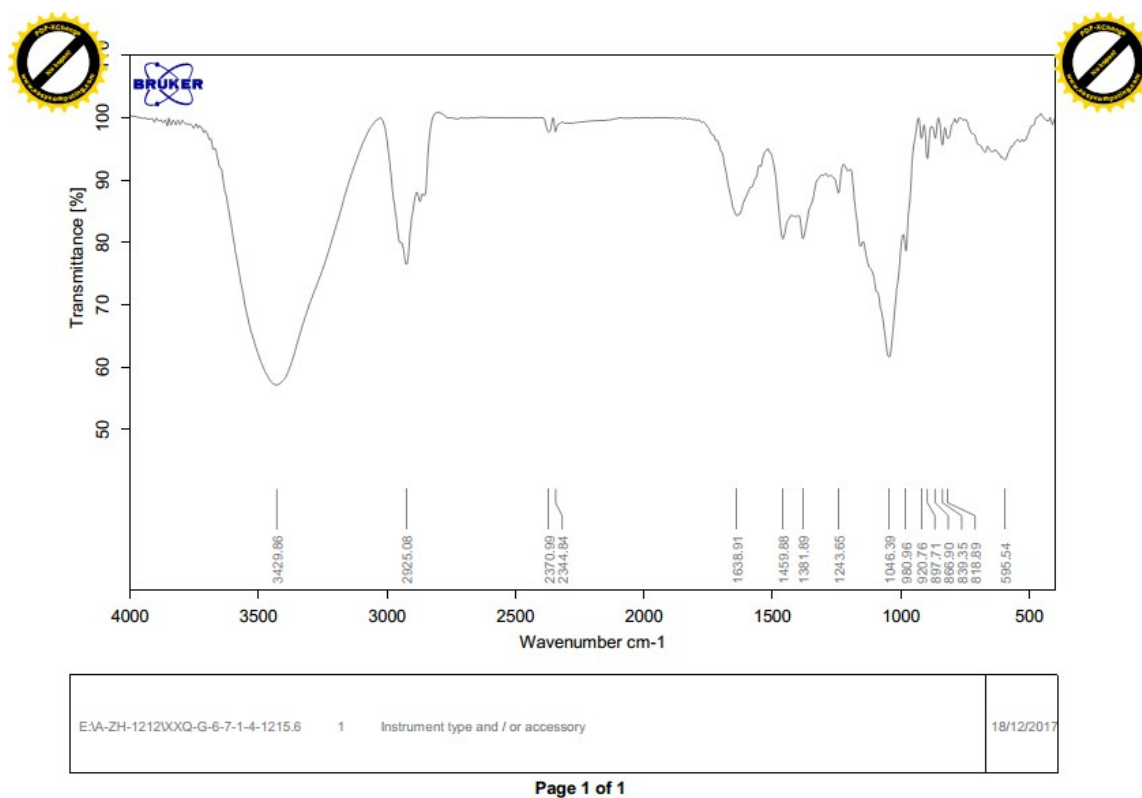
Figure S21. IR (KBr, disc) spectrum of compound 4
