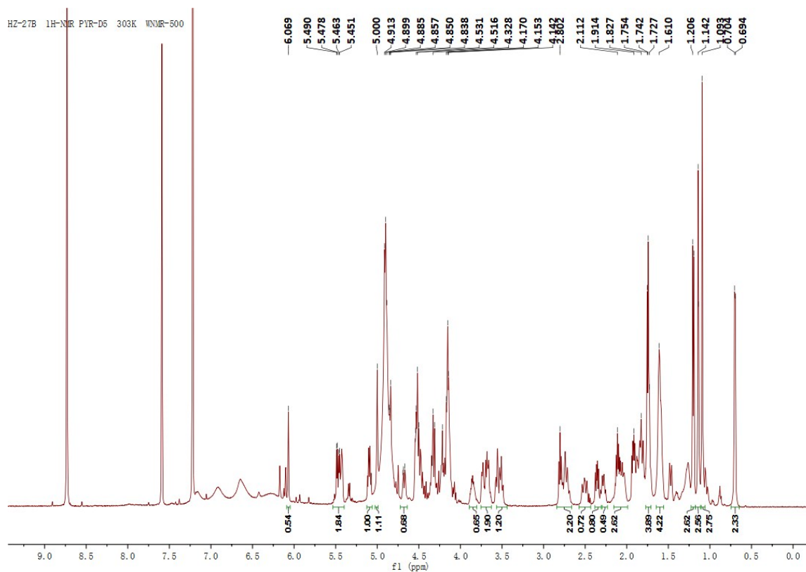
Figure S22. 1 H NMR spectrum of compound 4 (pyridine- d 5 )
