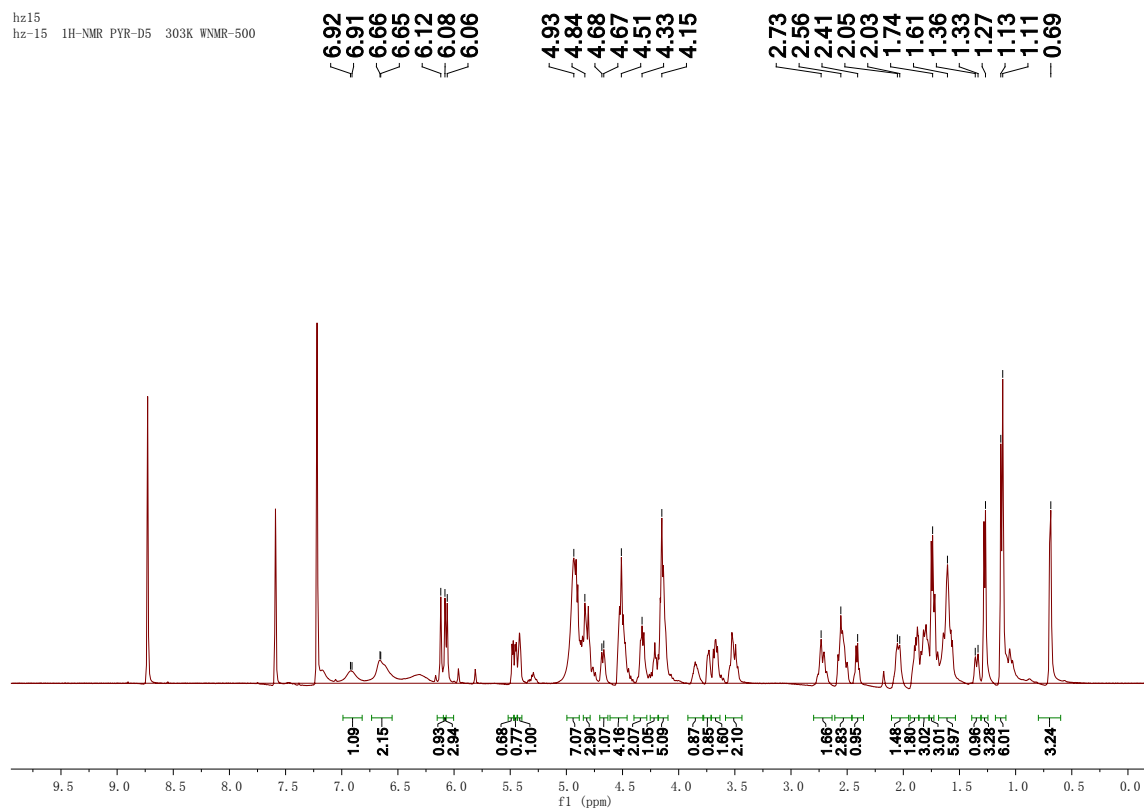
Figure S10. ^{13}\text{C} NMR spectrum of compound 2 (pyridine- d_5 )
