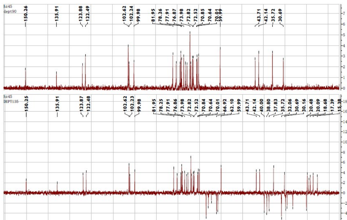
Figure S38. HSQC NMR spectrum of compound 6 (pyridine- d_5 )
