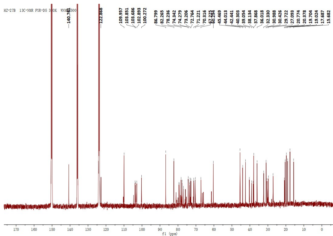
Figure S24. HSQC NMR spectrum of compound 4 (pyridine- d_5 )
