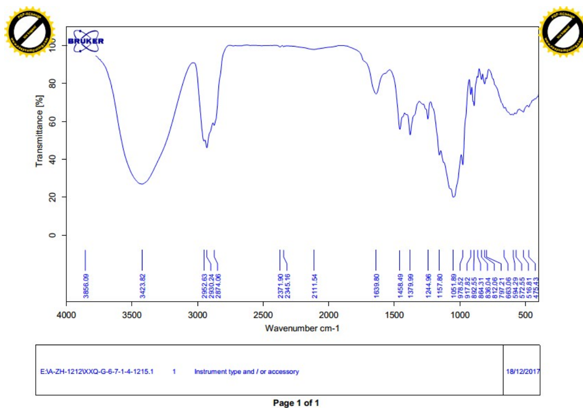
Figure S27. IR (KBr, disc) spectrum of compound 5
