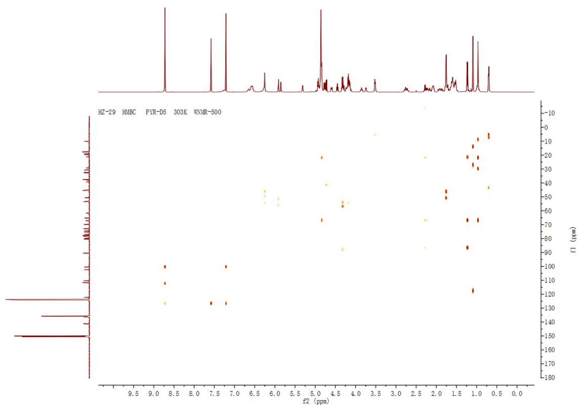
Figure S6. HMBC NMR spectrum of compound 1 (pyridine- d_5 )
