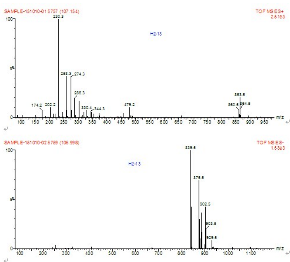
Figure S40. ESI-MS spectrum of compound 7
