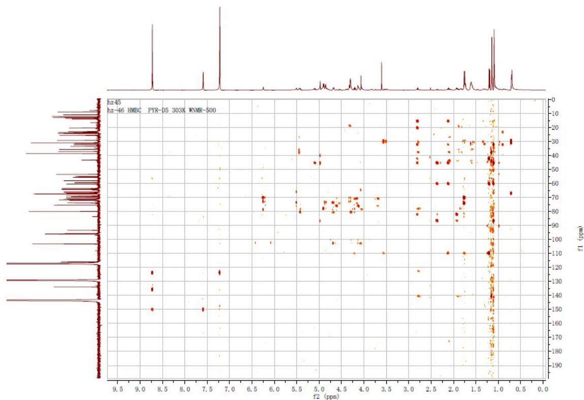
Figure S39. HMBC NMR spectrum of compound 6 (pyridine- d_5 )
