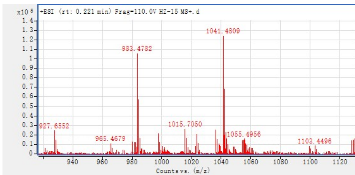
Figure S8. IR (KBr, disc) spectrum of compound 2
