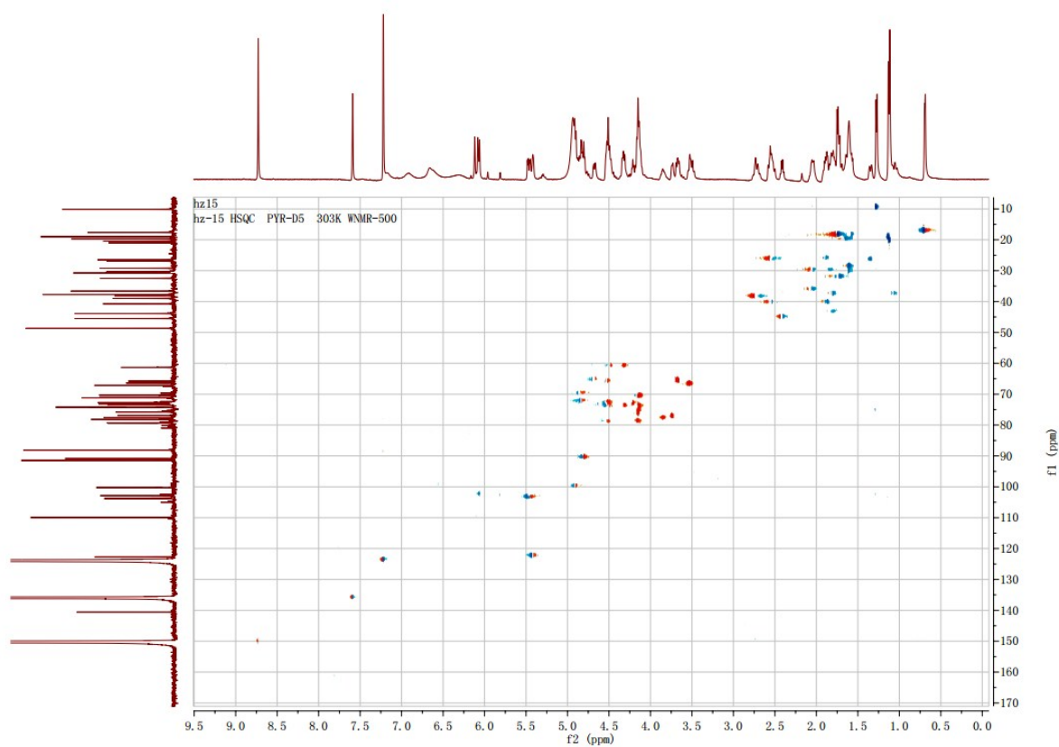
Figure S12. HSQC NMR spectrum of compound 2 (pyridine- d_5 )
