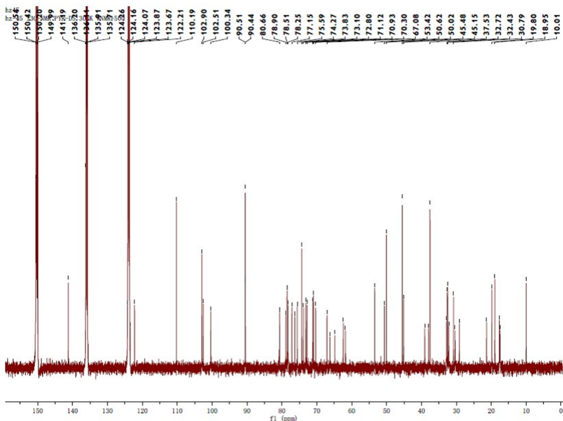
Figure S30. DEPT spectrum of compound 5 (pyridine- d_5 )
