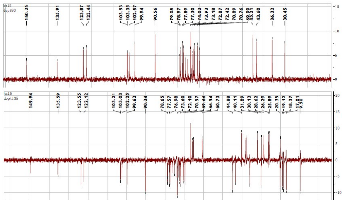
Figure S11. DEPT spectrum of compound 2 (pyridine- d_5 )
