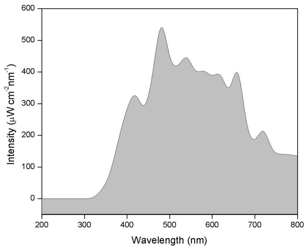
Fig. S1 .Emission spectrum of the visible light source provided by the supplier (OSRAMHCI-T 150 W/942 NDL PB)
