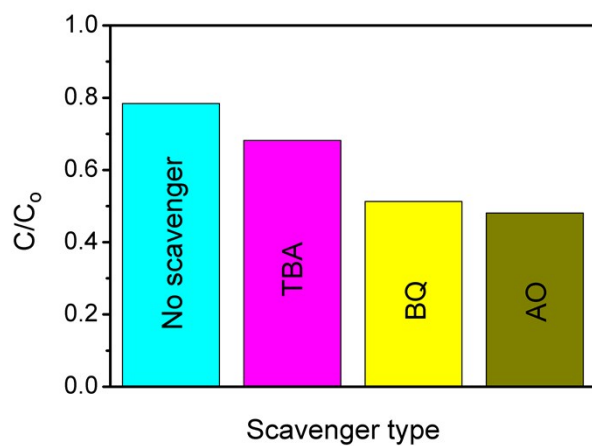
Fig. S2 The effects of various scavengers for the photocatalytic degradation of MB solution using ZnO-ZnS-3 for 75 min.
