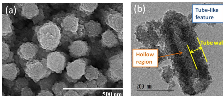
Fig. S1 (a) SEM image of the ZnO rods treated with 4-h sulfidation. (b) TEM image of the ZnO rod treated with 4-h sulfidation wherein the ZnO rod transformed into ZnS tube.
