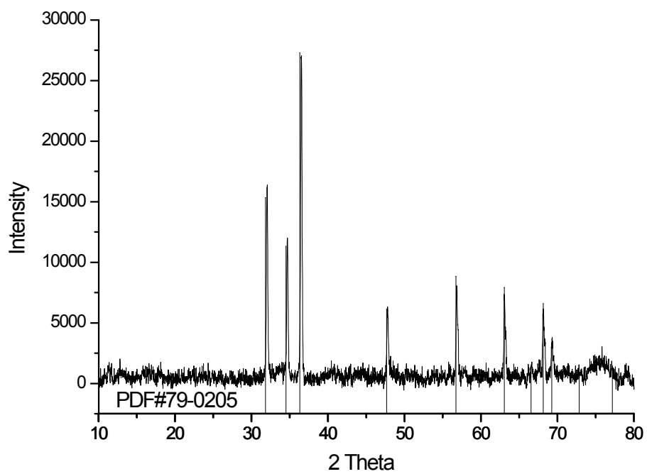
Fig. S13 XRD pattern of ZnO
