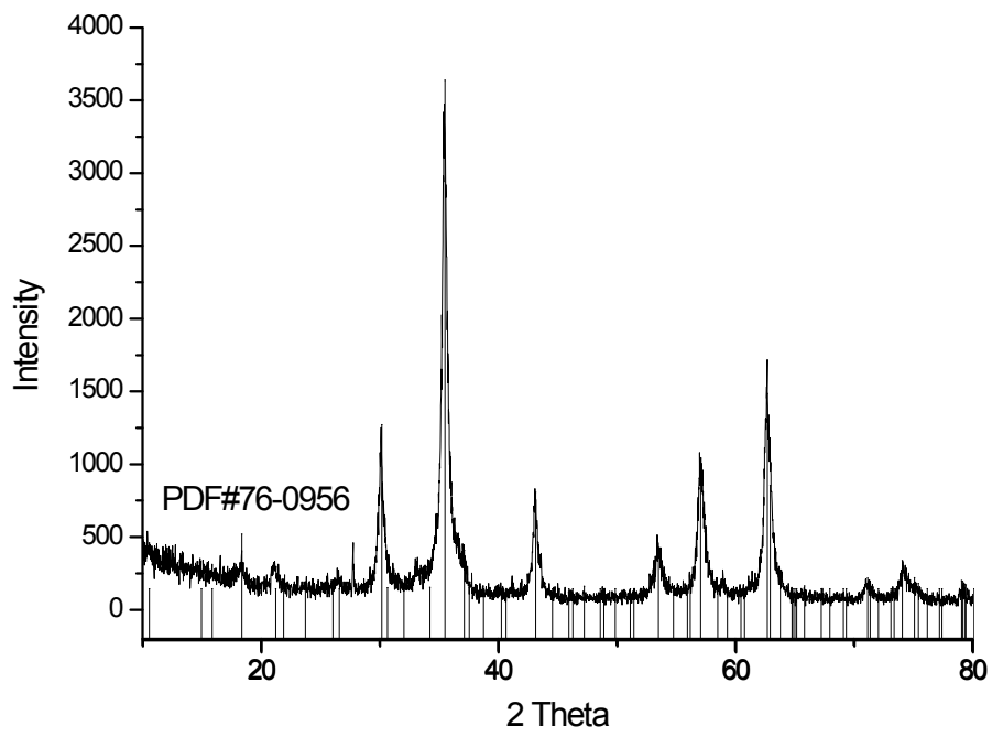
Fig. S15 XRD pattern of Fe 3 O 4
