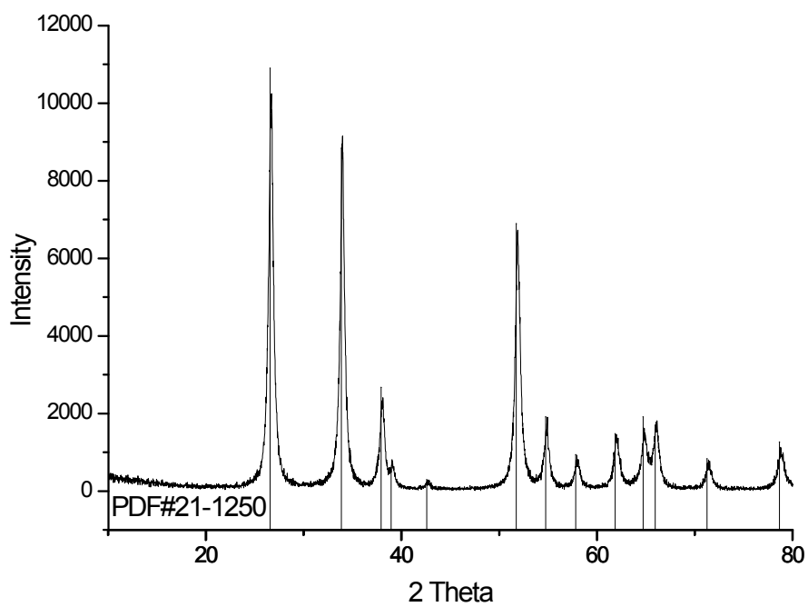
Fig. S14 XRD pattern of SnO 2
