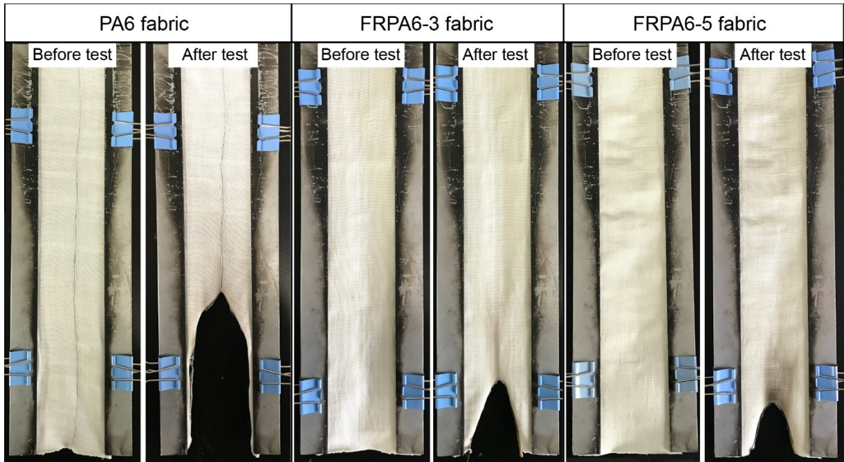
Figure S3. The photograph of PA6 and FRPA6 fabrics before and after vertical burning test
