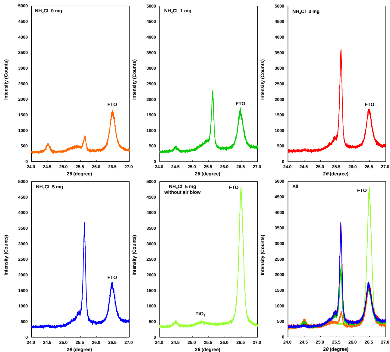
Fig. SI-4. Enlarged XRD peaks of FTO for the present cells.
