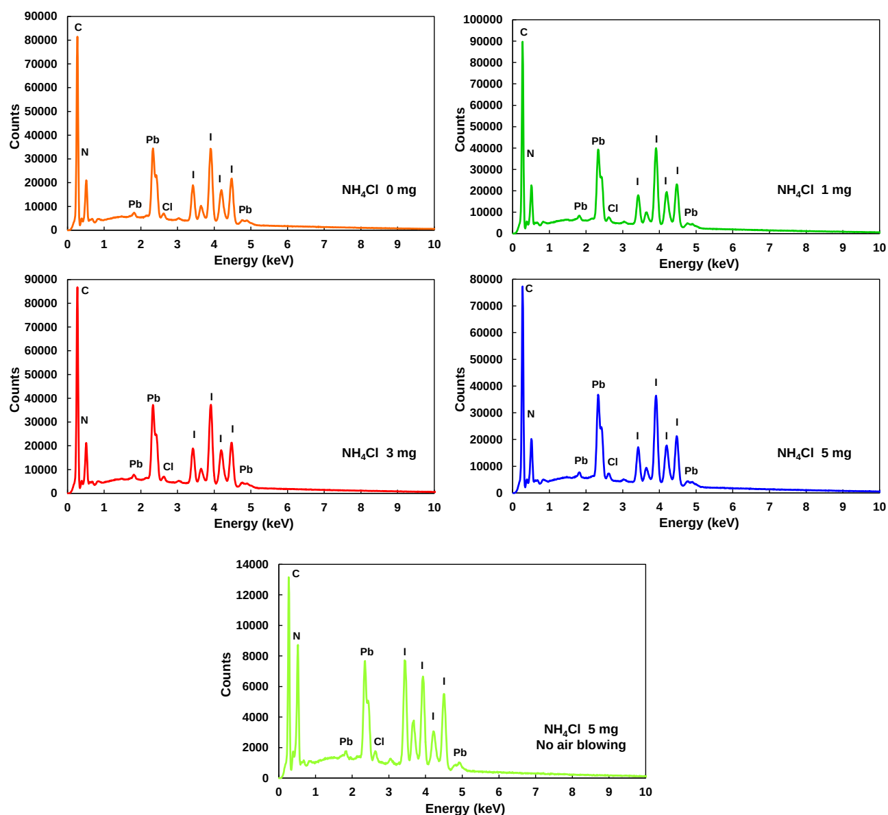
Fig. SI-1. Raw EDX data of the present cells.
