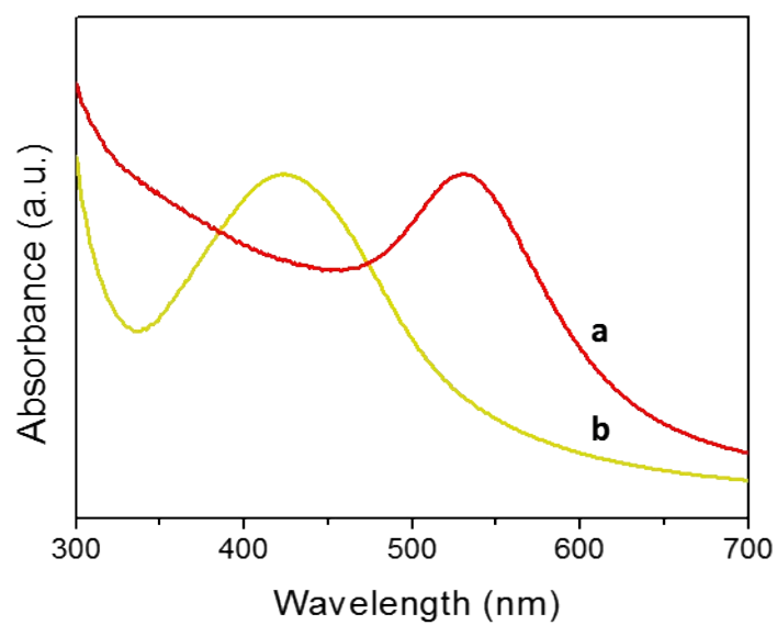
Figure S4. UV-Vis spectra of patchy micelles with NPs: (a) Au NPs; (b) Ag NPs.
