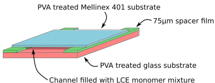
FIGURE S1 diagram of cell construction
