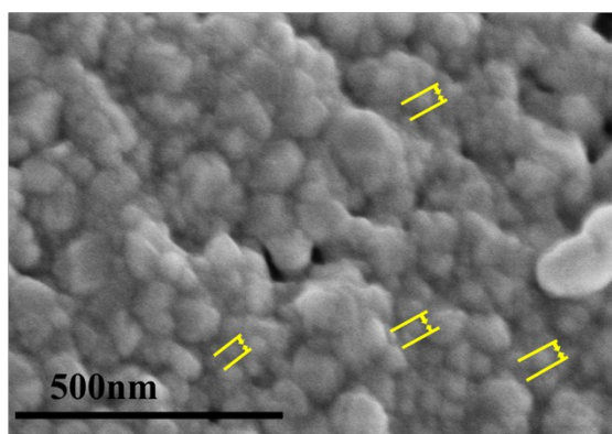
Fig. S2 SEM images of PET-PDA/Ag fabric
