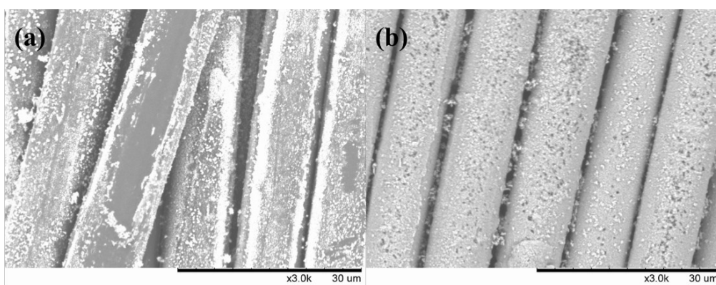
Fig. S1 SEM images of (a) PDA-PET/Ag fabric without immersing in the metal salt solution for activation and (b) PDA-PET/Ag fabric with immersing in the metal salt solution for activation.
