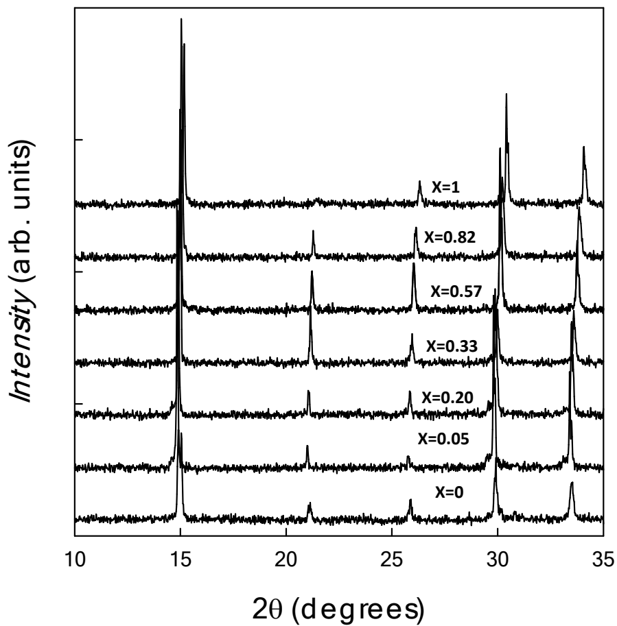
Figure 1. XRD patterns for the samples of the \text{FA}_{1-x}\text{MA}_x\text{SnBr}_3 system in the 10\text{-}35^\circ range. Patterns are vertically shifted to clarify viewing
