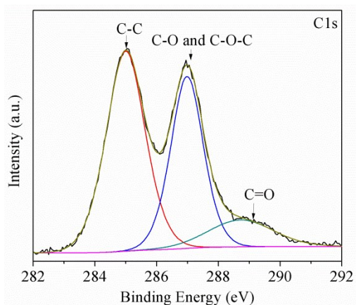
Figure S1. XPS spectra of C 1s for graphene oxide film.
