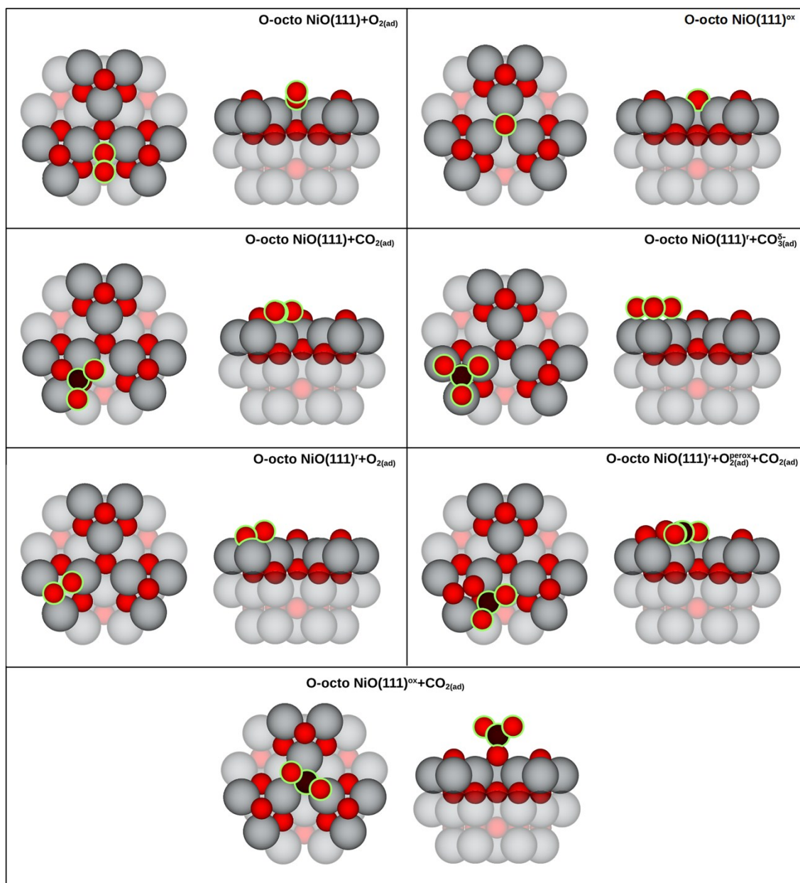
Fig. S1 Detailed geometries (top and size views) of adsorbed species involved in the proposed mechanism of the electrode reaction mechanism of cathode in the molten carbonate fuel cell
