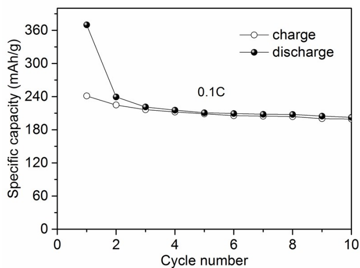
Figure S3. Cycling performance of TiO 2 -5d electrode at 0.1C.
