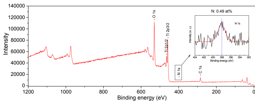
Figure S1. XPS spectra of TiO 2 mesocrystals.
