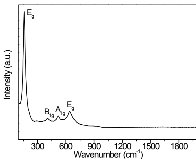
Figure S2. Raman spectrum of TiO 2 mesocrystal.
