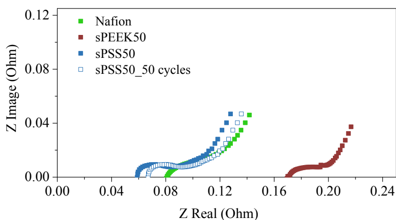
Figure S1. EIS curves of Nafion, sPEEK50, sPSS50 and sPSS50_50 cycles.
