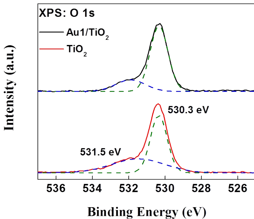
Fig. S1. XPS (a) Ti 2p and (b) O 1s spectra of TiO 2 and Au1/TiO 2 .
