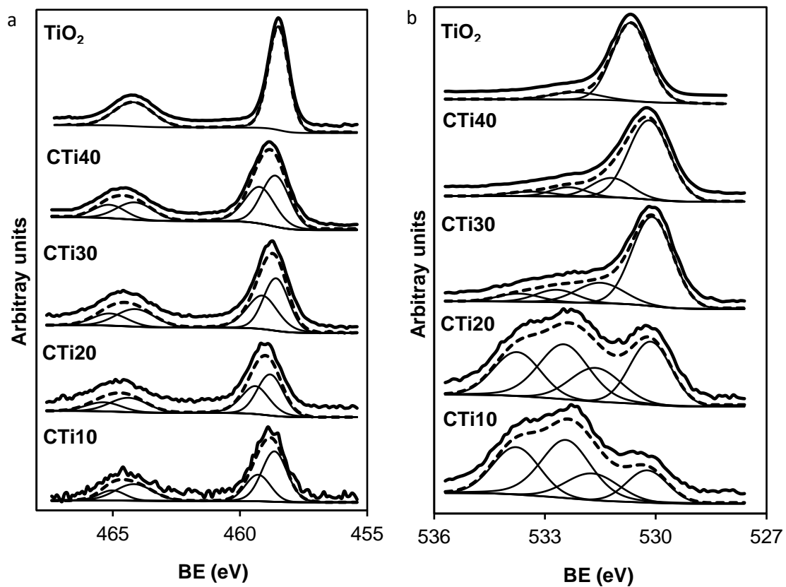
Figure S2. XPS spectra of \text{TiO}_2 -Carbon composites, a) \text{Ti}_{2p} and b) \text{O}_{1s} regions.
