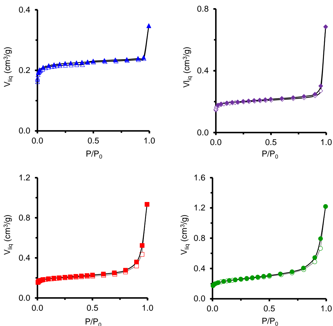
Figure S1. \text{N}_2 adsorption-desorption isotherms at -196\text{ }^\circ\text{C} on samples: CTi10 \blacktriangle , CTi20 \blacklozenge , CTi30 \blacksquare and CTi40 \bullet . Closed symbols: Desorption branch and opened symbols: Adsorption branch.
