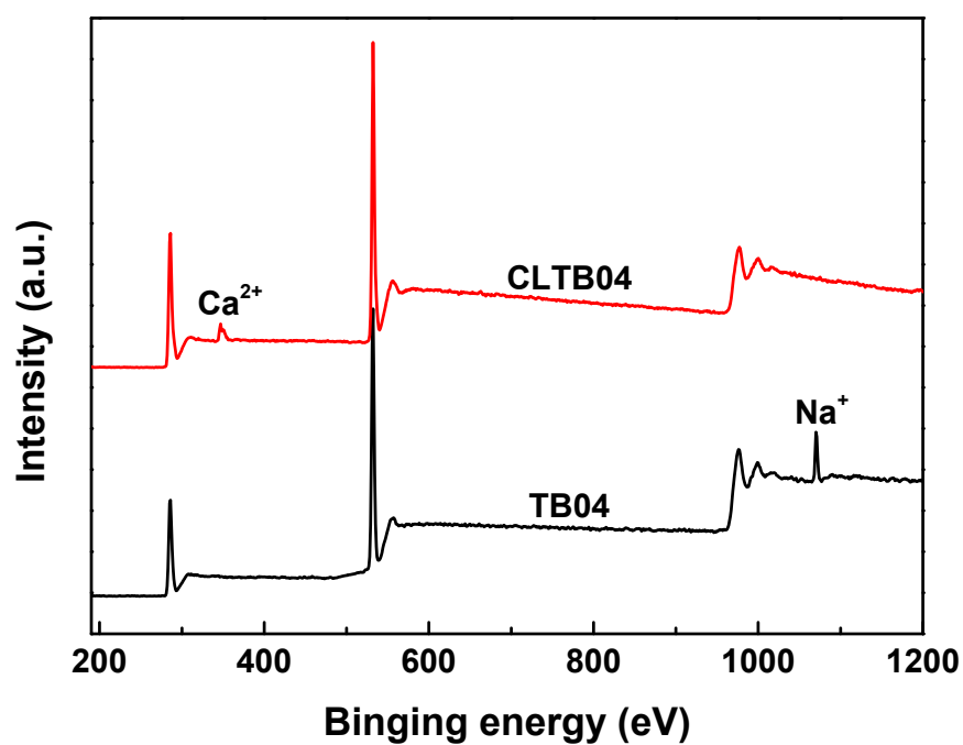
Fig. S1. XPS patterns of TB04 and CLTB04 films.
