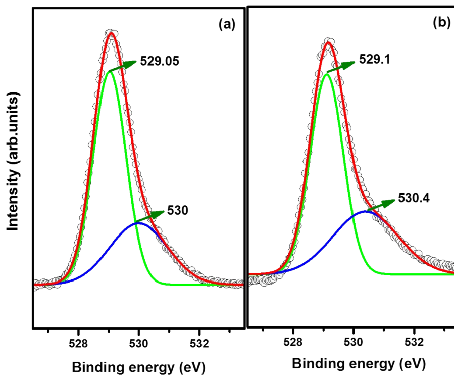
Fig: 1 O1s narrow scan spectra of 100 W deposited thin film taken a) immediately after deposition and b) 30 days after deposition.
