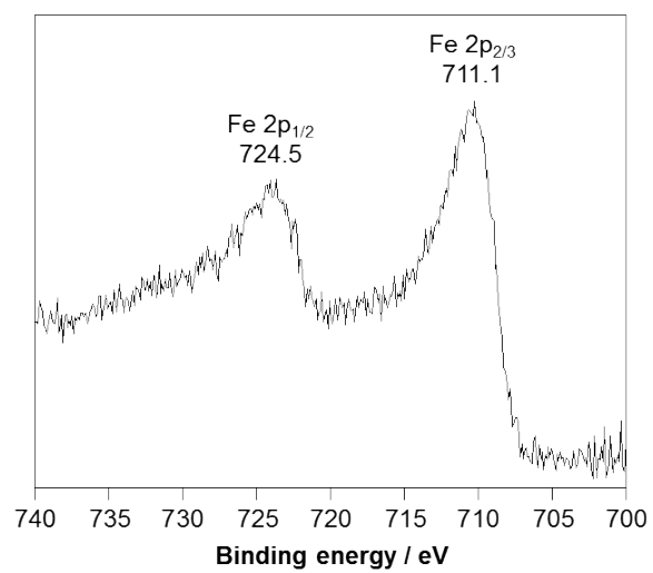
Fig. S2. XPS spectrum of Fe/HUS-7(120).
