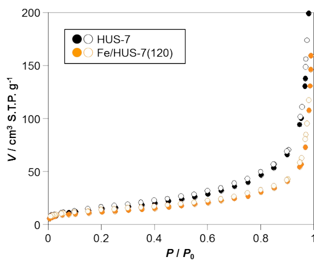
Fig. S3. N 2 adsorption (filled)/desorption(open) isotherms of HUS-7 and Fe/HUS-7(120). Prior to the measurements, the samples were evacuated at 80 °C for 12 h.
