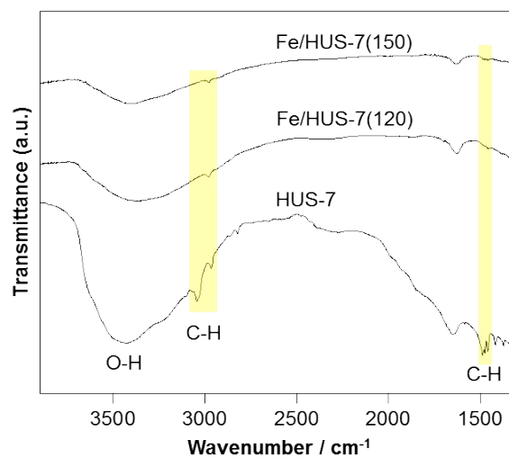
Fig. S1. FT-IR spectra of different samples.
