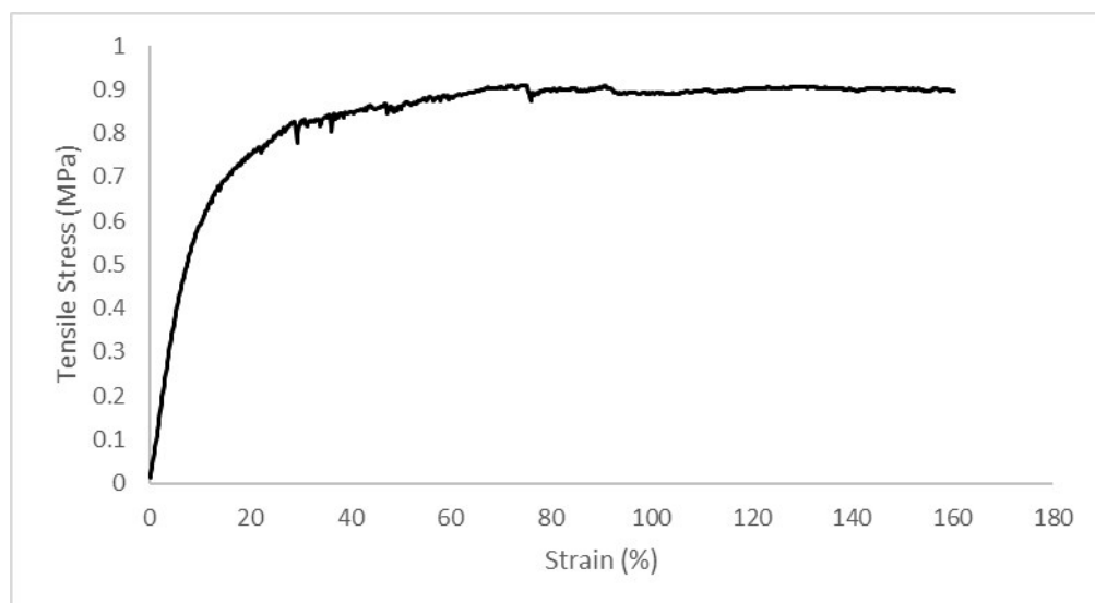
Figure S1: Stress-strain curve of PCL membrane
