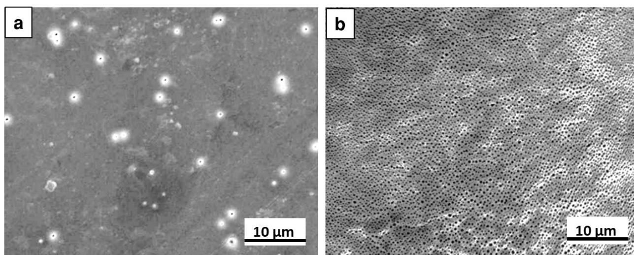
Figure S2: comparison between (a) commercial PET cell insert and (b) PCL membrane
