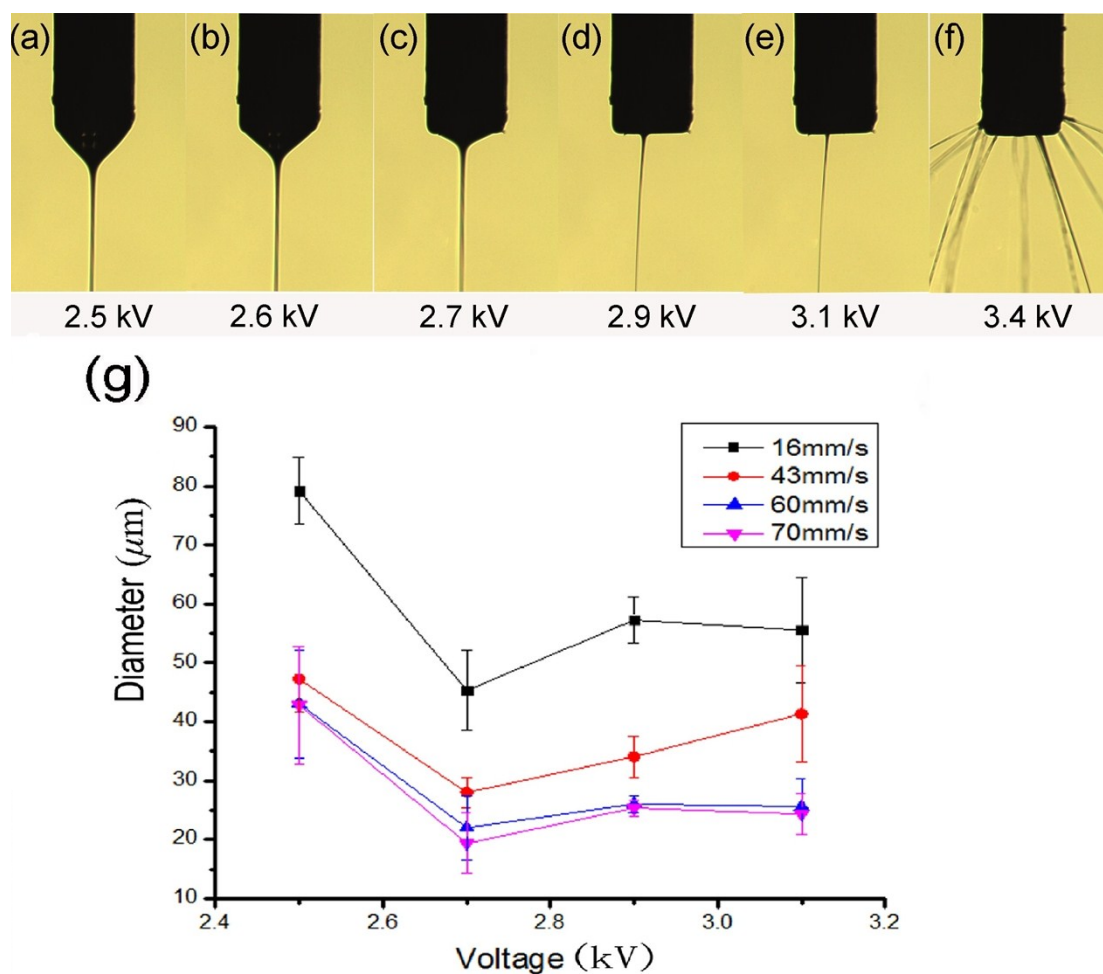
Fig. S1. E-jet printing process and printed filaments under different applied voltages (2.5–3.4 kV). (a–e) The shape of the jet changes with the increasing voltage. (f) Unstable multi-jets at high electric fields. (g) Printed filament width at different voltages using an 8% w/v PLGA solution.
