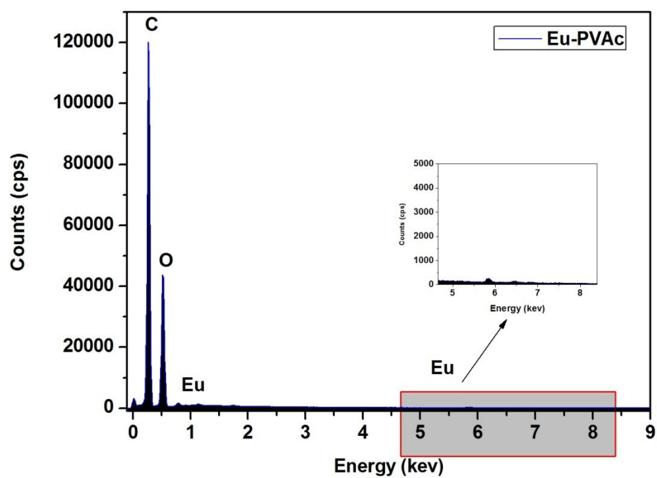
Fig. s4. EDS spectrum of Eu-PVAc
