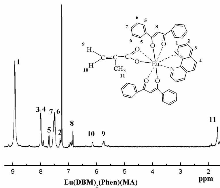
Fig. s2 ^1\text{H} NMR spectrum of \text{Eu}(\text{DBM})_2(\text{Phen})(\text{MA})
