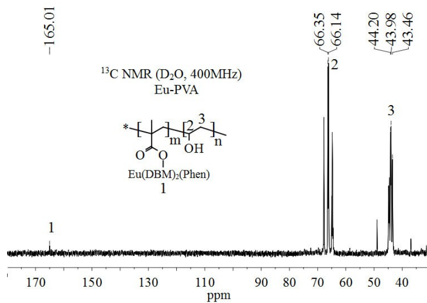
Fig. s3 ^{13}\text{C} NMR spectrum of Eu-PVA.
