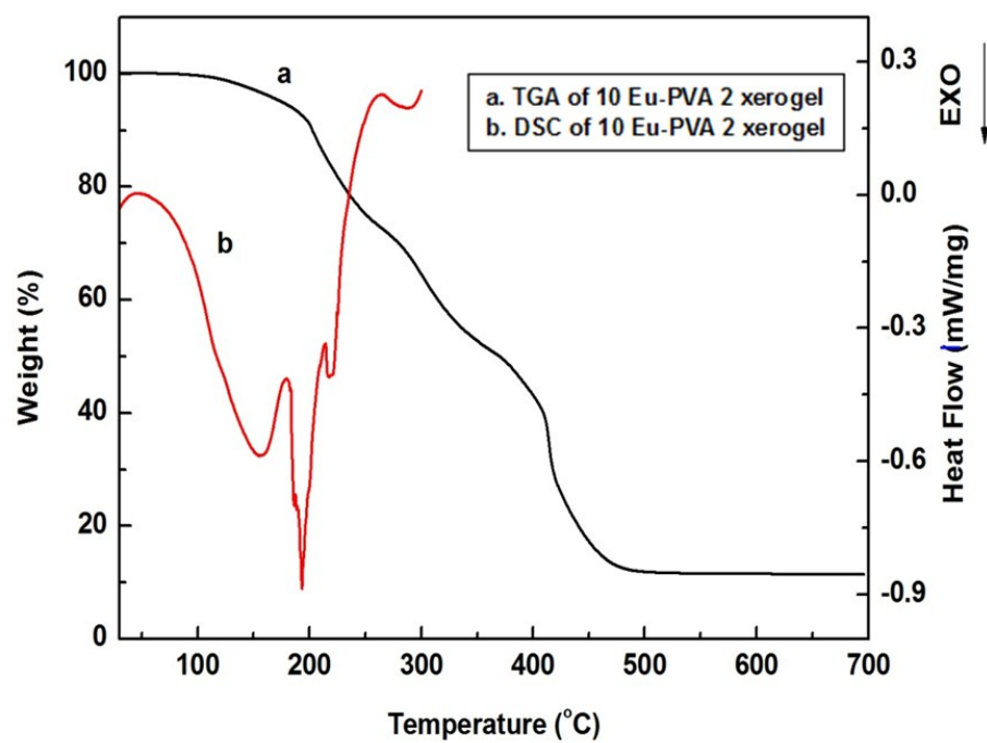
Fig. s5. (a) TGA curves of 10 Eu-PVA 2 xerogel, (b) DSC curves of 10 Eu-PVA 2 xerogel
