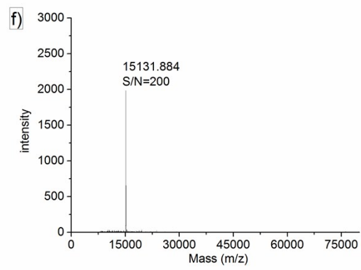
Fig. S1 MALDI-TOF spectra of BHb; A' standard of BHb; B' standard of CA; C' standard of SOD; A the bovine blood before adsorption; B the bovine blood after adsorption; e, f were eluents of e, f respectively.
