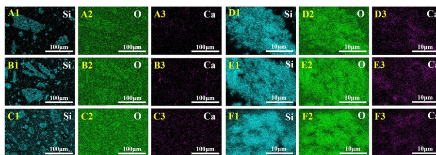
Figure. S1 The distribution of MCS in the resin matrix by EDS-mapping analysis. A1-A3, B1-B3 and C1-C3 images represent the distribution of MCS in the cross-section of 5RC, 10RC and 20RC, respectively; D1-D3, E1-E3 and F1-F3 images represent the distribution of MCS on the surface of 5RC, 10RC and 20RC, respectively. The distribution of MCS in the cross-section and on the surface of resin composites becomes dense and uniform with the increase of the amount of MCS nanoparticles.
