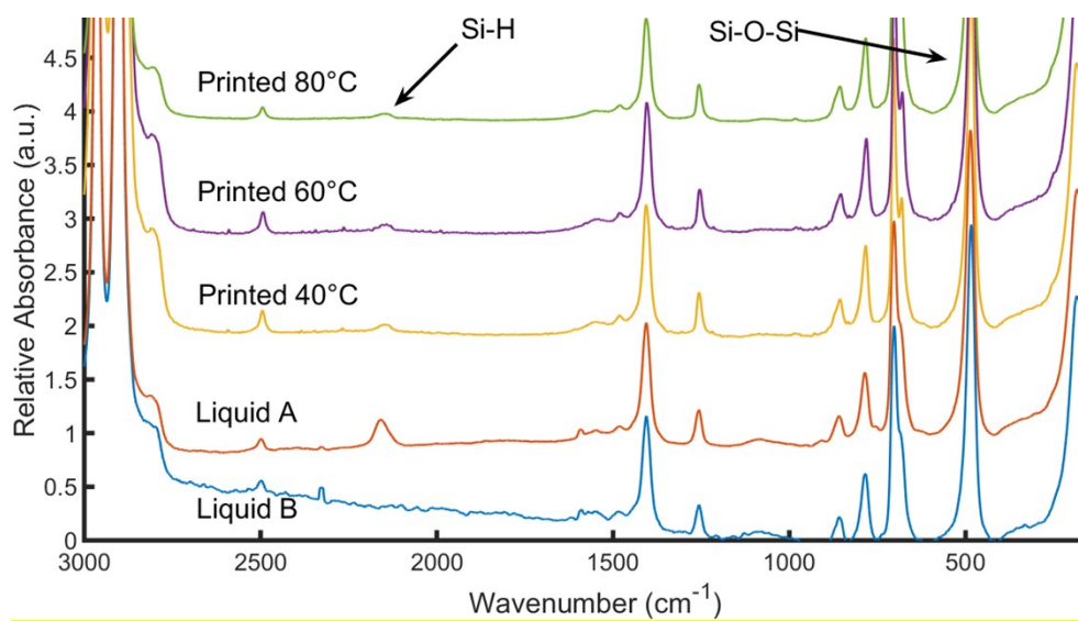
Supplementary 1 - Supplementary Information - Representative FTIR spectra for PDMS A, B and printed samples.
