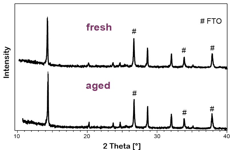
Figure S1. XRD spectra of freshly prepared perovskite absorber layer and aged samples
