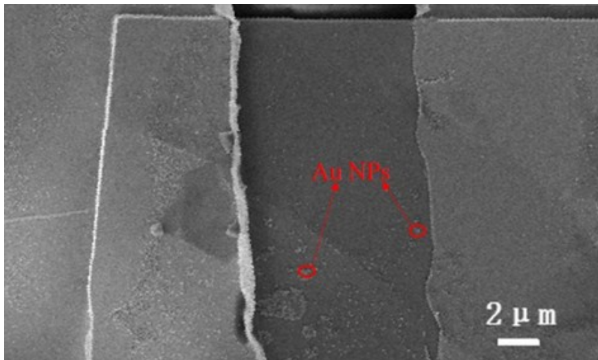
Figure S2. Au nanoparticles decorated the SnS nanosheet photodetector to form hybrid device.
