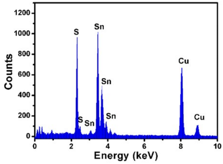
Figure S1. EDX spectrum recorded from the SnS nanosheets.
