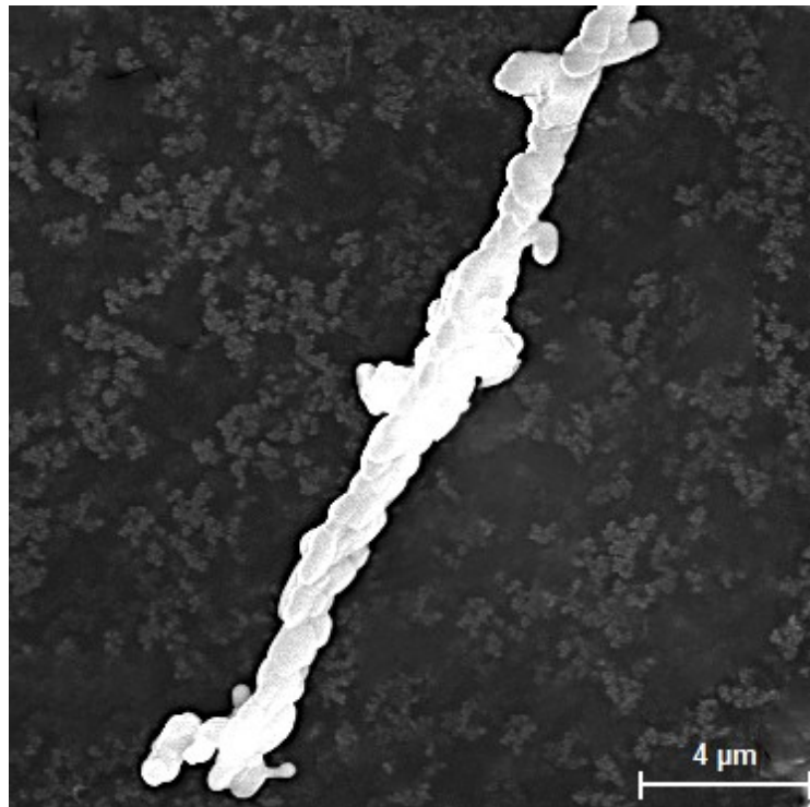
Fig. S3 SEM image of BNBT nanofibers annealed at 1000 °C for 6 hours.
