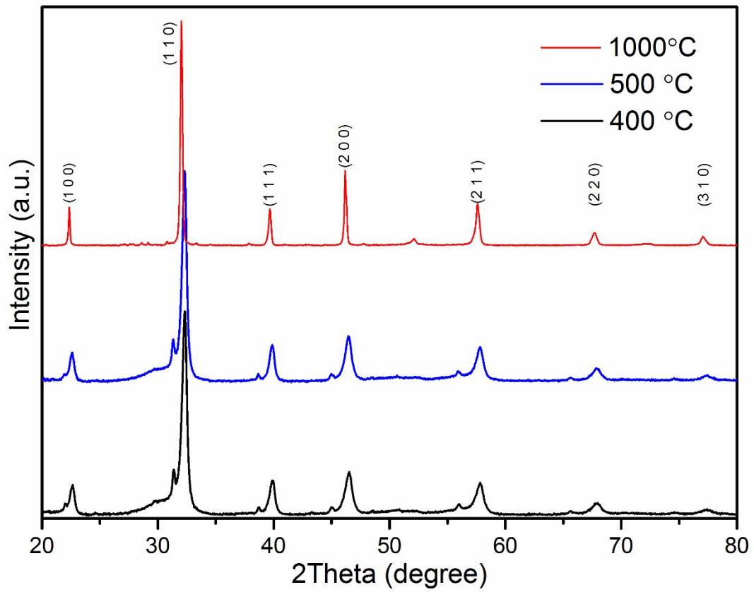
Fig. S2 XRD patterns of BNBT nanofibers annealed at different temperatures for 6 hours.
