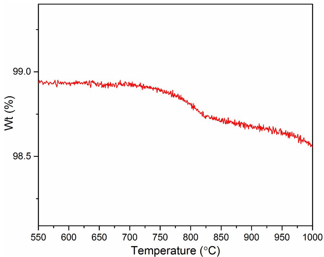
Fig. S1 TGA analysis of BNBT nanofibers.
