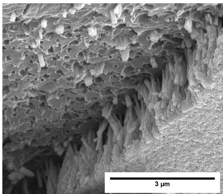
Figure S1 SEM image of the ZnO/PEDOT:PSS interface with ZnO partially removed. The holes in the PEDOT:PSS layer originated from the tips of the ZnO nanorods which penetrated inside the layer.
