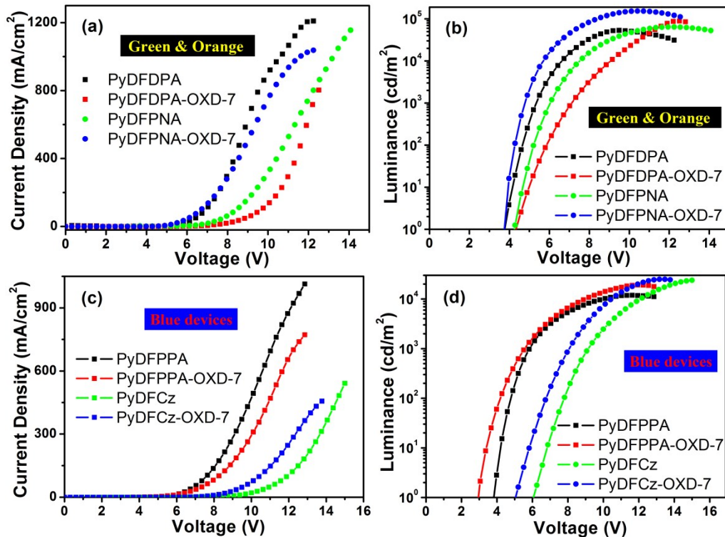
Fig. S2. Current density-voltage-luminance curves of the green, orange (a, b), and blue (c, d) OLEDs.
