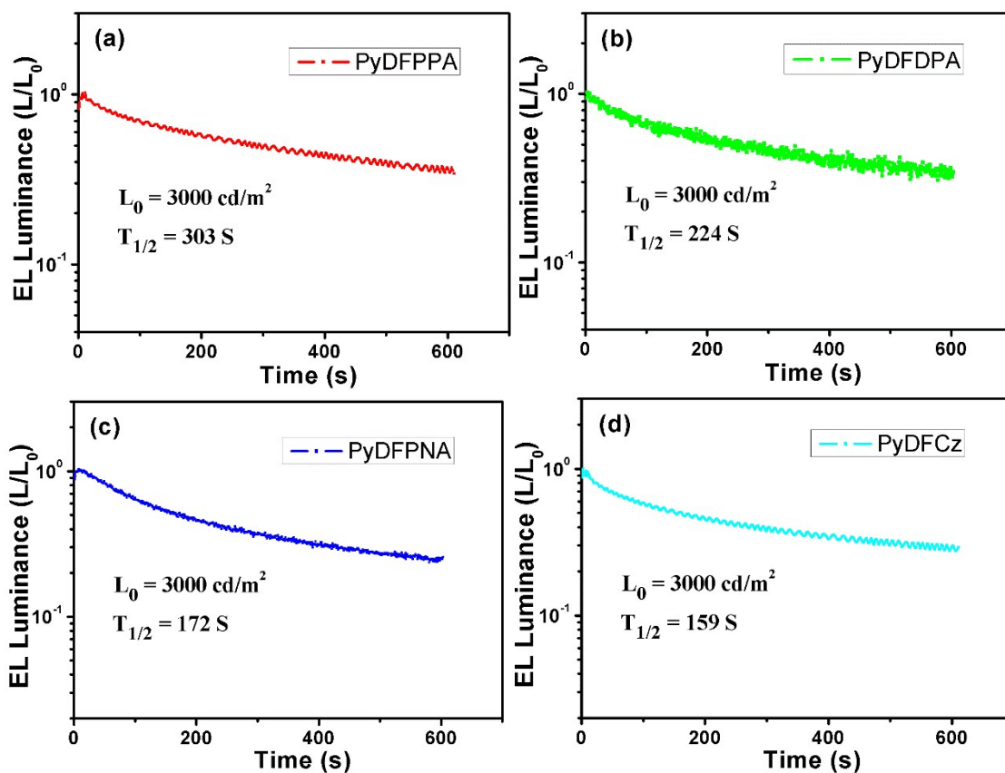
Fig. S4. Device operating lifetime of the blue, green, and orange phosphorescent devices based on PyDFPPA, PyDFDPA, PyDFPNA, and PyDFCz host at an initial luminance of 3000 cd m -2 under constant current mode.
