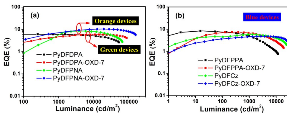
Fig. S3. EL efficiency versus luminance curves of the green, orange (a), and blue (b) OLEDs.
