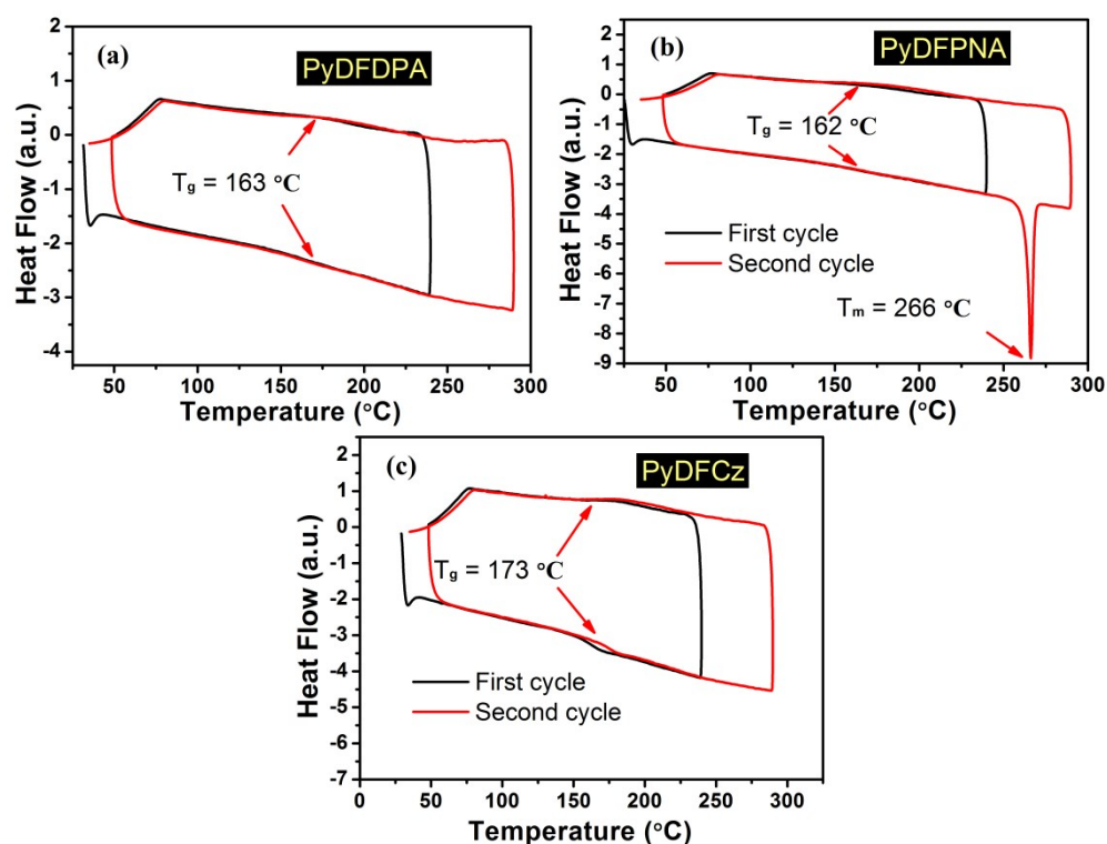
Fig.S1. The differential scanning calorimetry (DSC) curves of of PyDFDPA, PyDFPNA, and PyDFCz.
