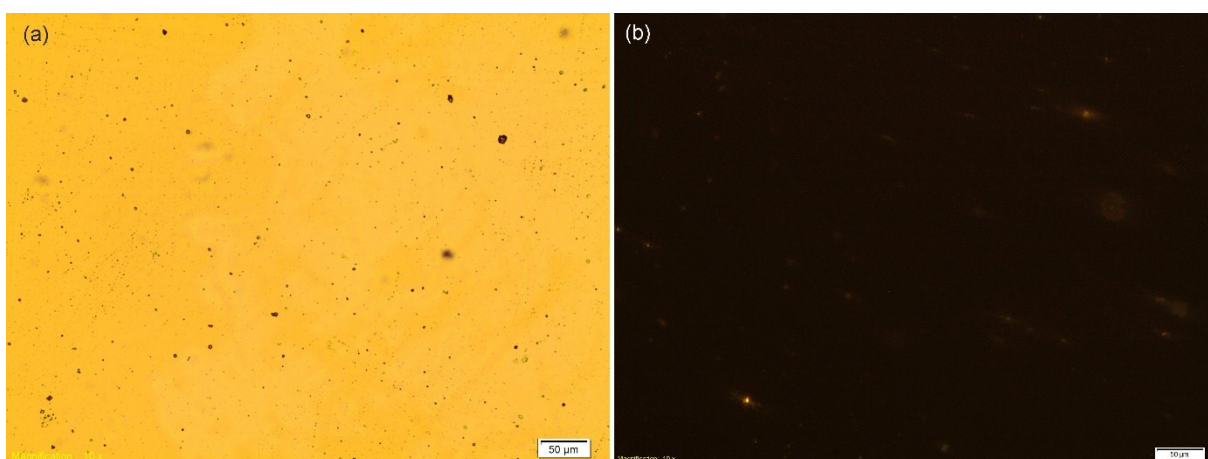
Fig. 2si. Optical microscopy images for TQPP-Me vacuum deposited thin film taken in polarized light (left) and in crossed polarized (right).
