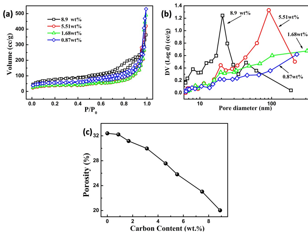
Fig. S2 (a) Nitrogen adsorption-desorption isotherm, (b) pore-size distribution and (c) open porosity of metacomposites with different carbon contents.
