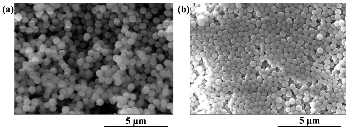
Fig. S1 SEM images of (a) SiO 2 powder and (b) neat SiO 2 bulk sintered at 800 °C for one hour.
