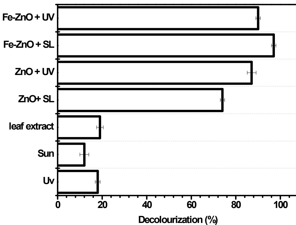
Figure S1. Percentage decolourization of 50 ppm Indigo carmine dye using 25mg/L of ZnO and Fe-doped ZnO, NPs at 4 h under sunlight and UV.
