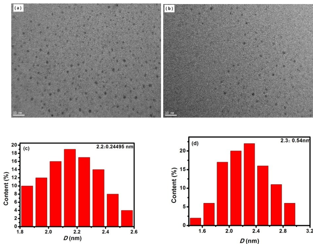
Fig. S1 TEM images of TGA -CdTe QDs (a) and MPA-CdTe QDs (b). Diameter distributions of TGA -CdTe QDs (c) and MPA-CdTe QDs (d).
