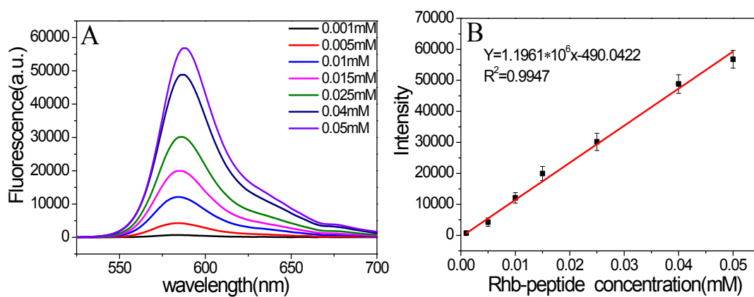
Fig. S1 (A) Fluorescence emission spectra of the Rhb-peptide after excitation at 355 nm. (B) Calibration curve for intensity at 580 nm versus varying concentrations of Rhb-peptide after excitation at 355 nm.
