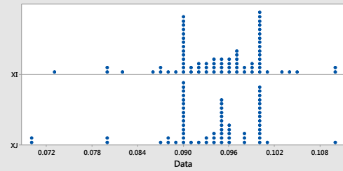
MgO
