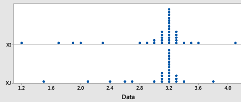
MgO
