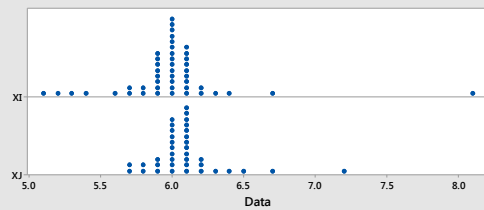
CaO
