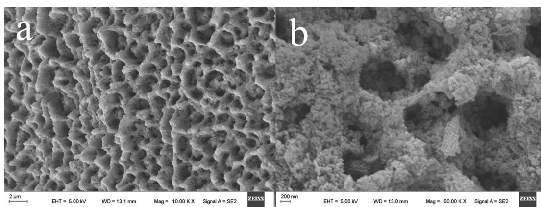
Fig. S2 SEM micrographs (a \times 10000 and b \times 50000) of the Ti-TiO 2 MPs@HANPs fiber after soaking in organic solvents for 24 h.
