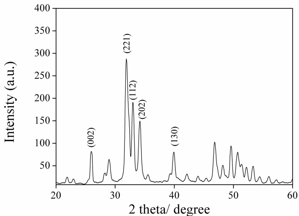
Fig. S1 XRD pattern of HANPs.
