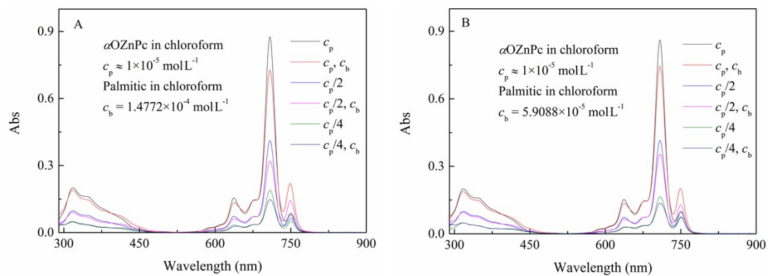
S1. UV-vis spectra of concentration-different \alpha OZnPc in chloroform with and without palmitic acid, which has two concentrations 1.4772 \times 10^{-4} \text{ mol/L} (a) and 5.9088 \times 10^{-5} \text{ mol/L} (b).
