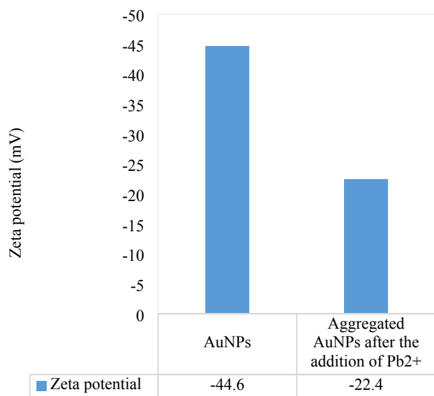
Fig.S3 Zeta potential over the addition of Pb 2+ during the sensing procedure.
